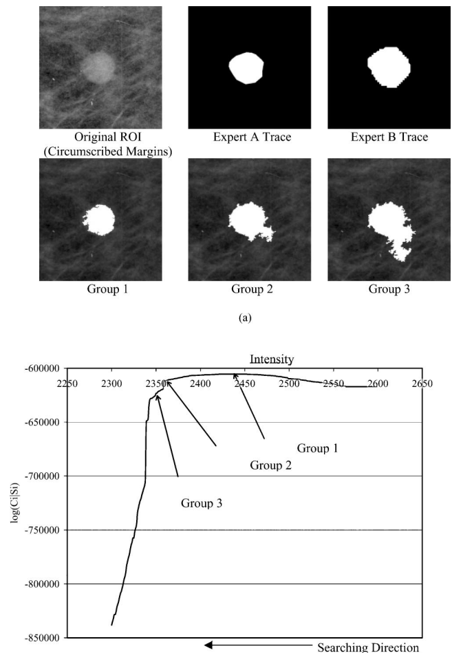
Fig. 6. (a) Segmentation results for a benign mass with circumscribed margins (subtlety=4); (b) the corresponding cost function.
