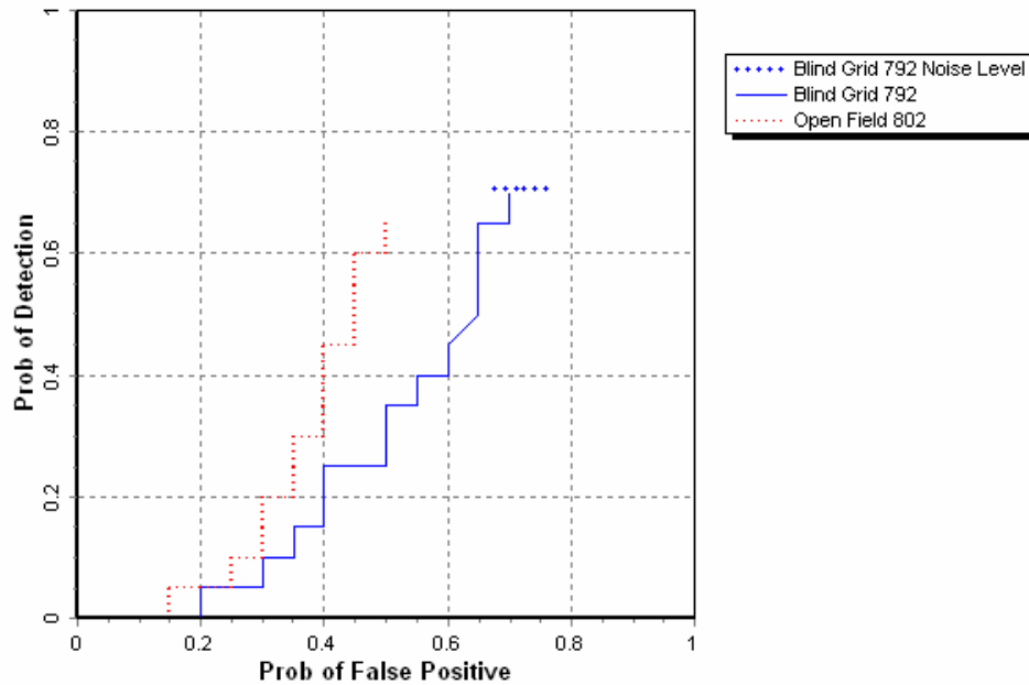
Figure 16. VSEMS dual/towed P_d^{\text{res}} versus the respective P_{fp} for ordnance larger than 20 mm.
