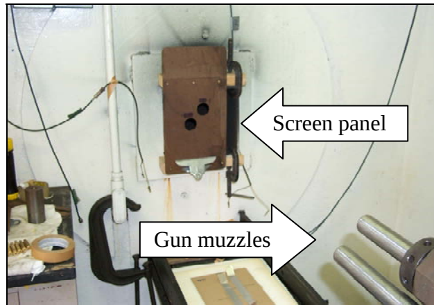
Figure 14. Front make-screen mounting panel.
