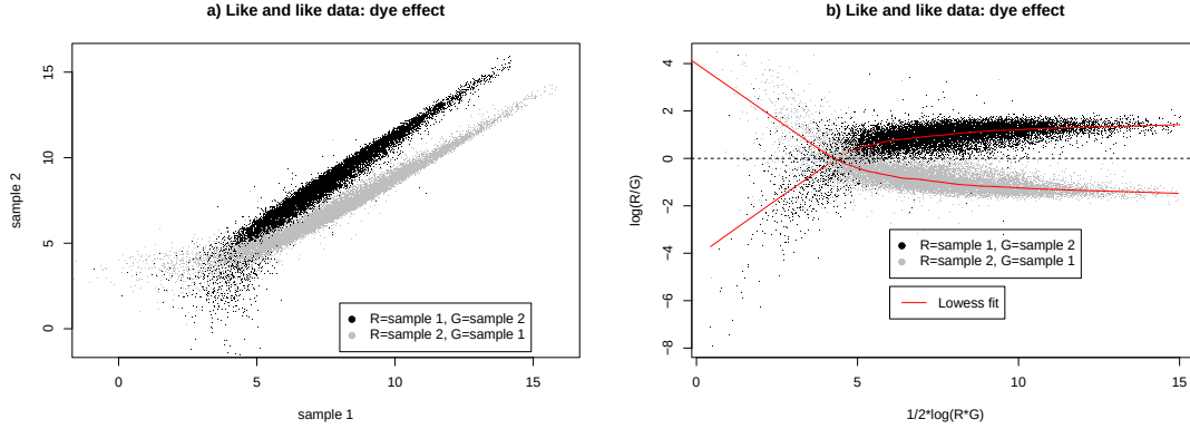
Figure 1: Effect of the Dye Swap on the Like and Like Data. (a) \log(\text{sample 1}) versus \log(\text{sample 2}) . This shows that the dye effect is approximately additive on the log scale. (b) Overall intensity versus log ratio. This shows that the non-linear effects will approximately cancel one another out in a balanced dye-swap experiment. The overall intensity is half the sum of the log intensities in the two channels, and all logarithms are to base 2.
