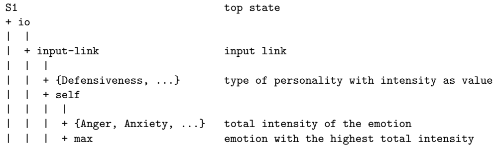
Figure 4.2: Tree structure of the locations in the input link
