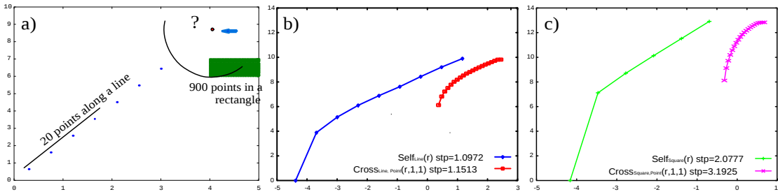
Figure 12: Classifying a point as either belonging to a sparse line or to a dense square, using the cross-cloud method: (a) spatial placement of the incoming point and the datasets, (b) Self_{Line}(r) and Cross_{Line,Point}(r,1,1) plot, (c) Self_{Square}(r) and Cross_{Square,Point}(r,1,1) plot.
