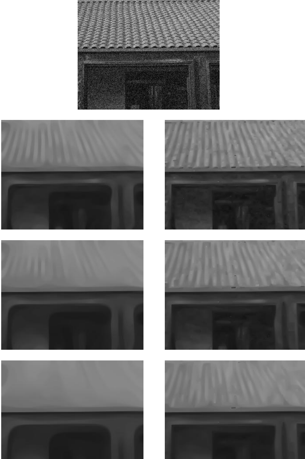
Figure 3.15: Top: House; Left: Geometric heat flow u_t = u_{\xi\xi} , (top to bottom) t = 40, 80, 160 ; Right: Flow u_t = \cos^2(2\theta) u_{\xi\xi} , (top to bottom) t = 40, 80, 160 .
