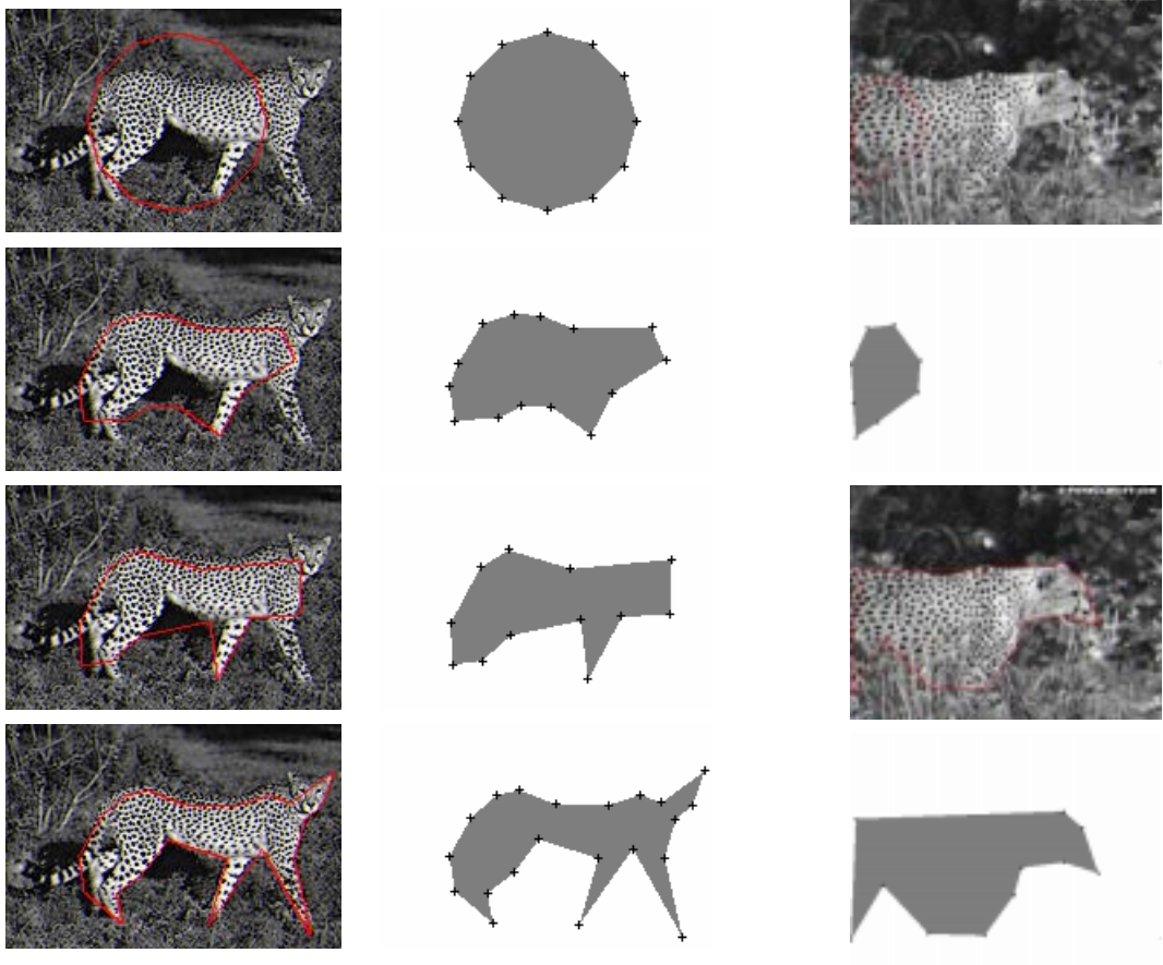
Figure 4.15: Left: Cheetah figure is captured by the active polygon. Right: A cheetah in bushes is captured with an active polygon.
