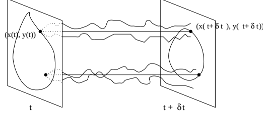
Figure 3.1: Illustration of averaging behaviour. Points of the zero-level set, i.e. initial contour (\mathcal{X}(t), \mathcal{Y}(t)) , at time t , is shown on the left. Those points whose sample realizations result in an average value of zero at time t + \delta t ( u(t + \delta t, \mathbf{x}) = E^{\mathbf{x}}[u(\mathbf{X}(t))] = 0 ) form the new contour (\mathcal{X}(t + \delta t), \mathcal{Y}(t + \delta t)) (on the right).
