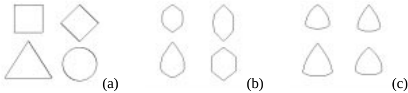
Figure 3.7: (a) Initial set of shapes (b) Flow \mathbf{C}_t = \cos^2(3\theta)\kappa\mathbf{N} , which tends to produce hexagons, (c) Flow \mathbf{C}_t = \sin^2(1.5(\theta - \pi/2))\kappa\mathbf{N} , which tends to produce triangle-like shapes.
