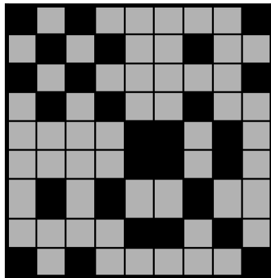
Figure 2 - Another example of BVD as clustering the proximity matrix
