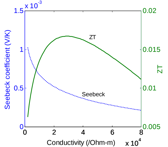
Figure 1: Seebeck coefficient and ZT as a function of the electrical conductivity for bulk crystal Silicon at 373K.
