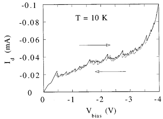
FIG. 3. The dark current-voltage characteristics for increasing bias scan (thick line) and decreasing bias scan (thin line) at T = 10 K.
