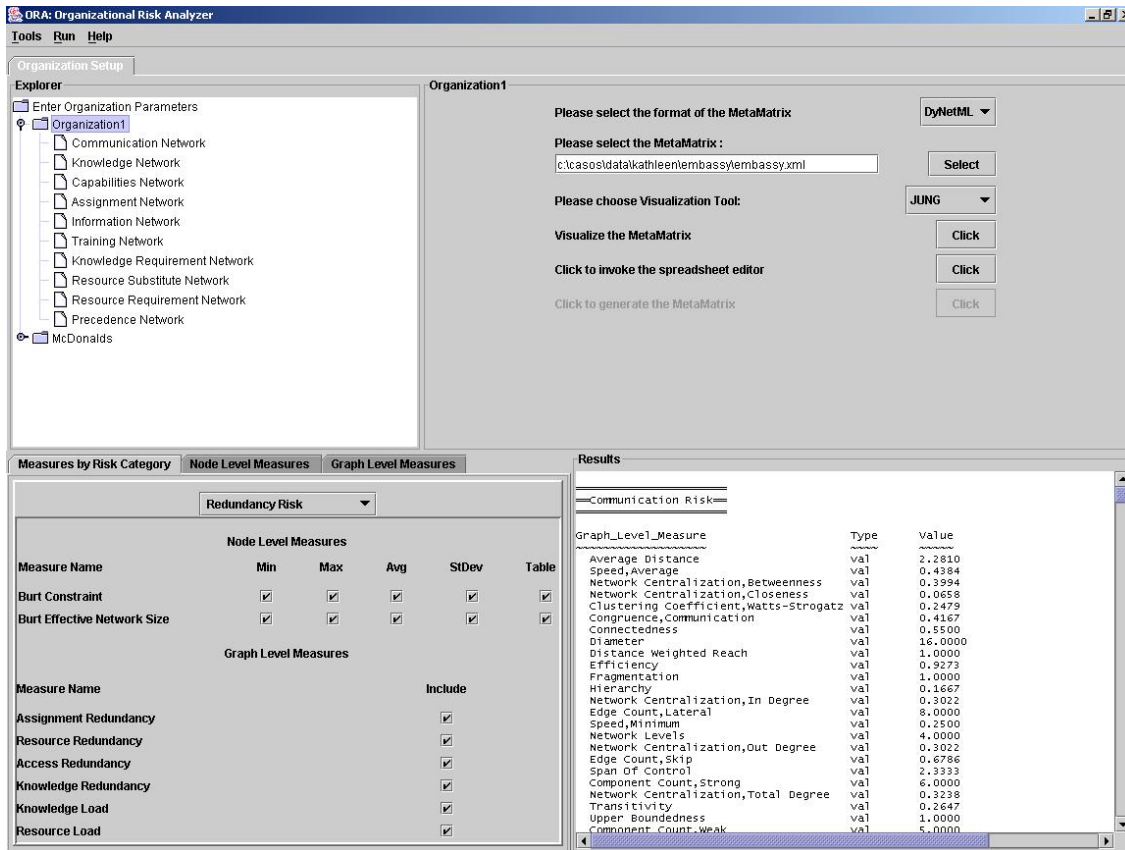
Figure 2 : ORA/Optimizer Interface
