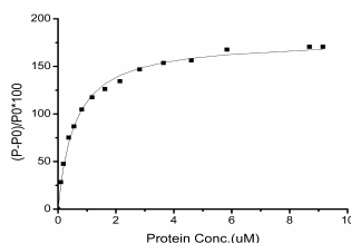
Figure 3. Competition Assay for Bid1le peptide using Fluor-Bid1l probe . Buffer: 20mM Phosphate pH 7.2, 50mM NaCl, 2mM DTT, 1mM EDTA 0.01% BGG.
