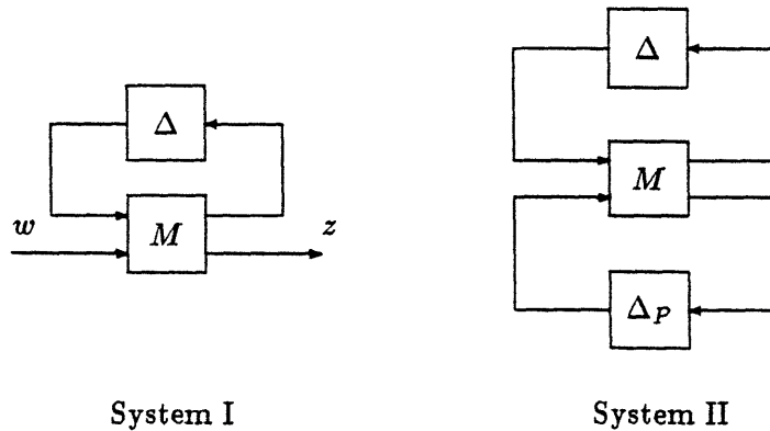
Figure 2.8: Stability Robustness vs. Performance Robustness
