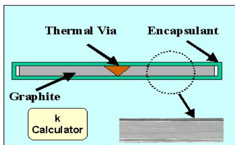
Figure 6: k-Technologies Patented k-Core Material System 10
