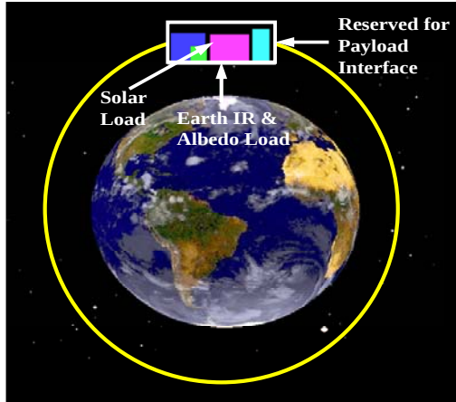
Figure 2: Worst Hot Case Orientation
