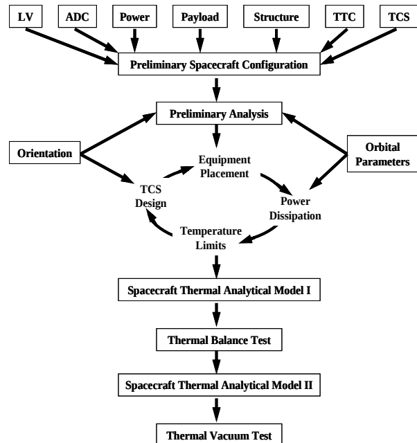
Figure 1: Overall Thermal Design Process
