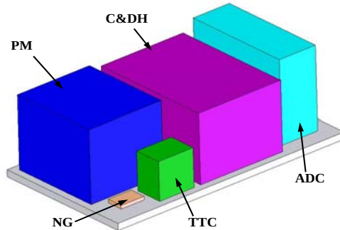
Figure 4: Layout of the LCB
