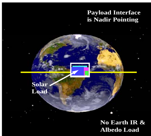
Figure 3: Worst Cold Case Orientation
