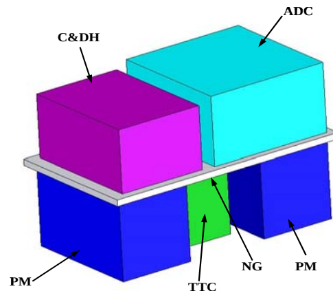
Figure 5: Layout of the HCB
