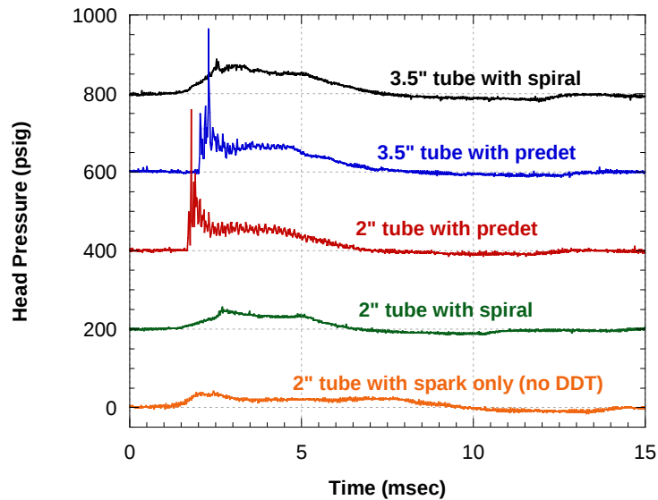
Figure 8. Head pressure traces versus time. Times are normalized to spark discharge and each pressure is offset 200psi for clarity.
