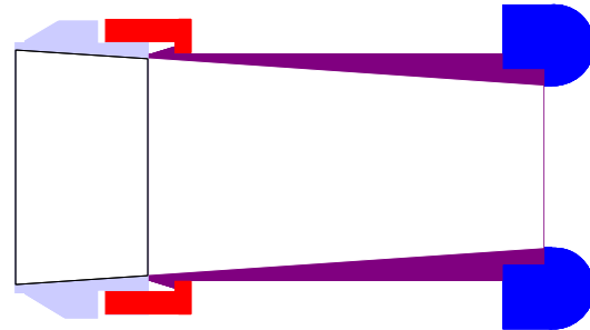
Figure 13. Straight and tapered ejector profiles used in the small scale pulsejet experiment of Ref. 3.
