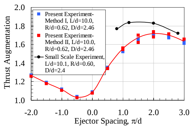
Figure 7. Thrust augmentation as a function of driver-to-ejector spacing for the D/d=2.46, L/d=10.0 ejector.
