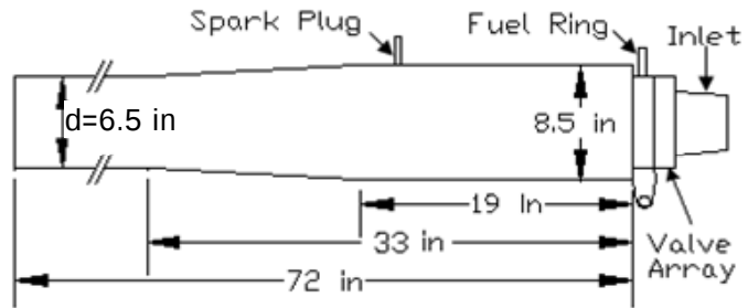
Figure 2. Pulsejet schematic.
