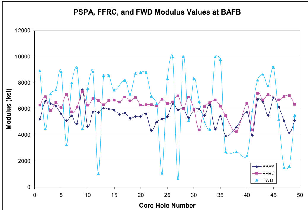
Figure 14. Modulus value trends at BAFB.
