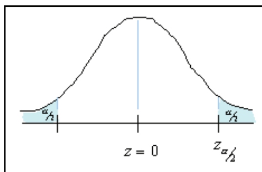
Figure 22. Sample distribution curve (iSixSigma 2000-2005).
