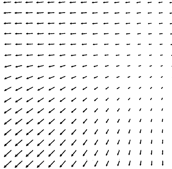
Figure 17: SOR algorithm flow estimates: R = 500^2 , 250 iterations. The SOR algorithm required a factor of 60 more computation in this example.
