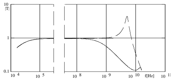
Fig.5. Frequency response of E-field probe without- (dashed line) and with RC filter.
