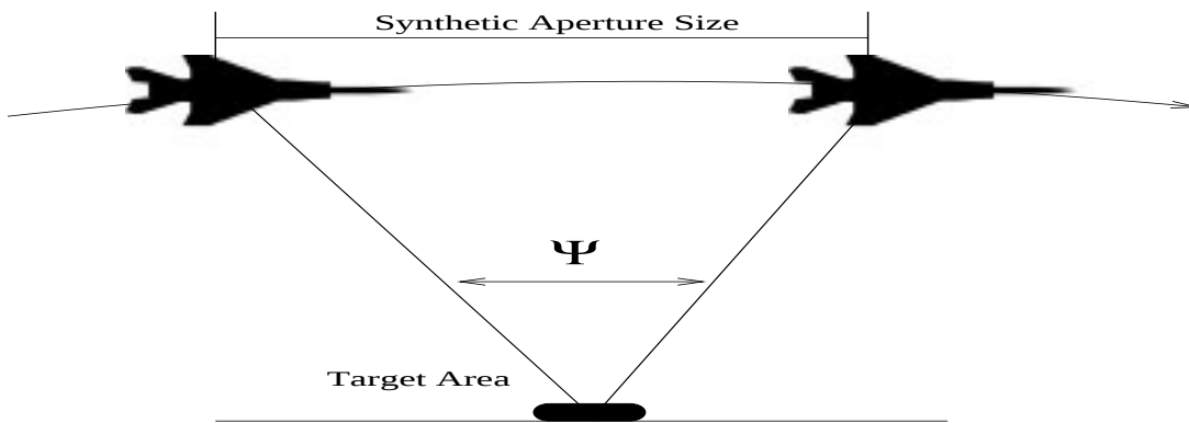
Figure 2.1: Spotlight SAR
