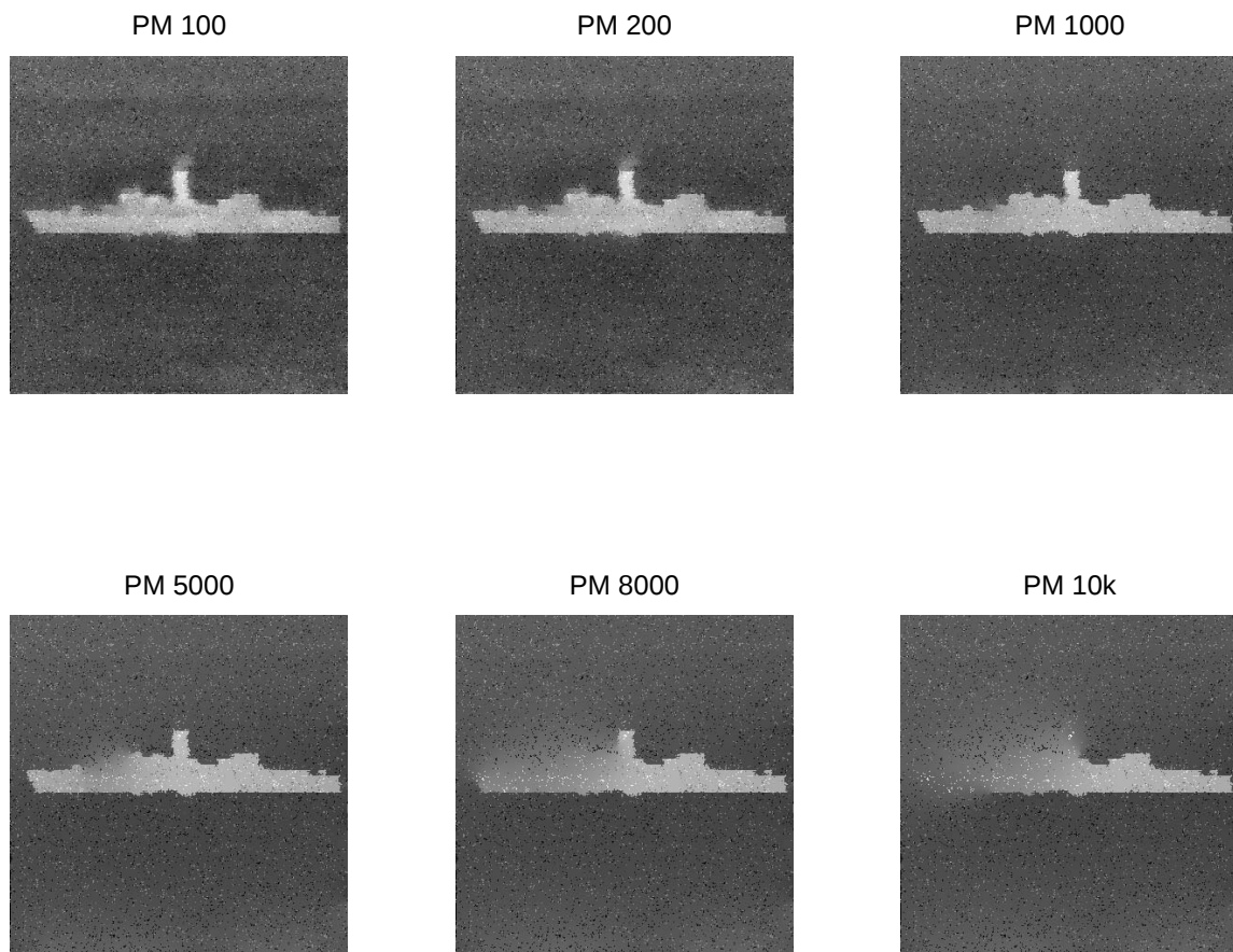
Figure 3.6: PM algorithm.
