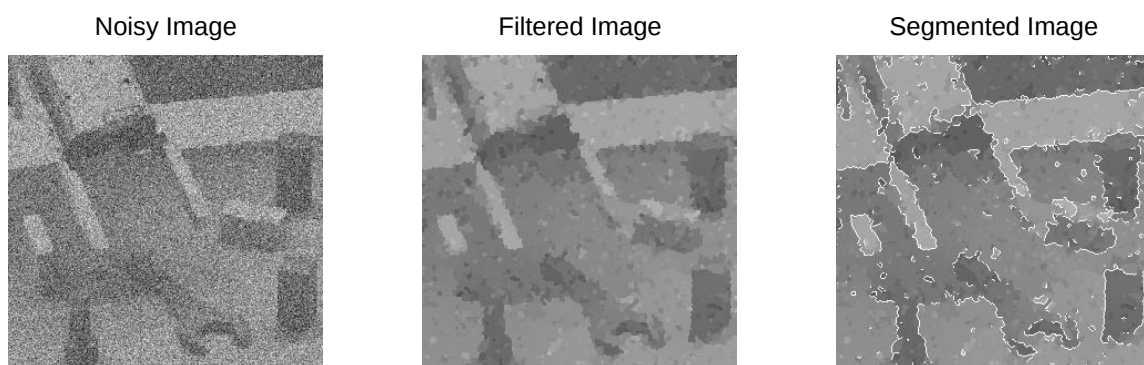
Figure 3.8: tools segmentation.
