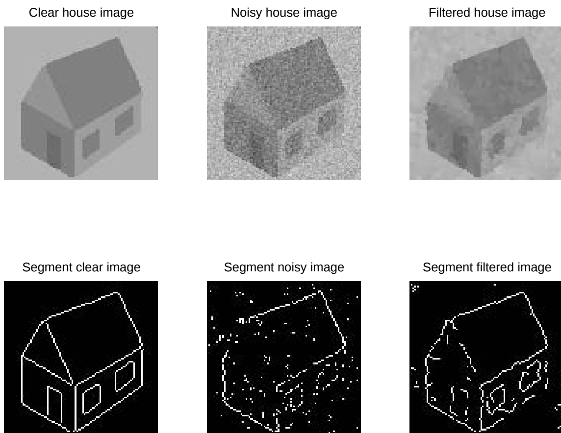
Figure 3.9: House segmentation.
