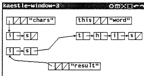
Figure 5-5: Illustration of the Validity of a Rule Using KAESTLE
