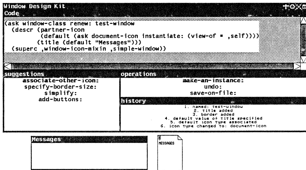
Figure 4-2: The Window and its Associated Icon
