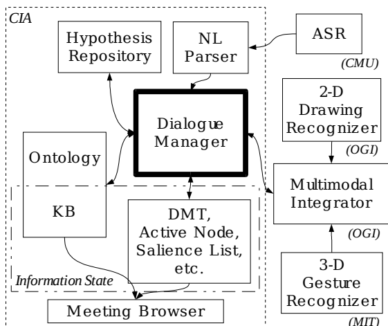
Figure 1: The meeting assistant architecture, highlighting the dialogue-management components.
