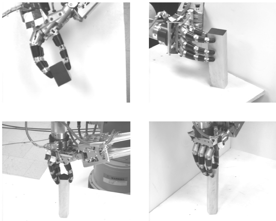
Fig. 5. Grasps synthesized by PICK-AND-PLACE and executed using a Utah/MIT hand. The top row shows two perspectives of the lateral grasp of a rectangular prism, while bottom row shows the overhand grasp of a pentagonal prism.
