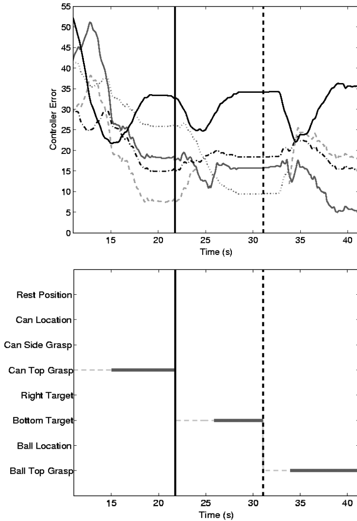
Fig. 14. Top: the graph shows the controller errors for five affordances over a portion of the demonstration. During this period of the experiment, the teleoperator grasped the can and released it on the bottom target in Fig. 13. Next, the arm was moved to grasp the ball. The affordances shown in this graph correspond to a rest position of the arm above the table (solid black line on top for a majority of the trial), the top grasp of the ball (solid grey), placing an object on the bottom target (dotted), placing an object on the right target (dot-dash), and a top grasp of the can (dashed). The controller errors for other affordances are not shown here. The solid vertical line shows the time at which the teleoperator performs a top grasp of the can. The corresponding affordance becomes unavailable shortly thereafter; this is shown by the line disappearing. The release of the can is shown by the dashed vertical line. After releasing the can on the bottom target, its affordance becomes unavailable, and the can affordance becomes active again. Bottom: the graph shows the estimated intended action extracted by the system (solid) and the true intended action (dashed) of the teleoperator, over the same period of the experiment. Grasp and release by the teleoperator is denoted as in the top graph.
