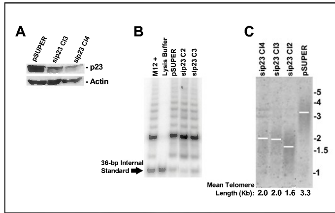
Figure 3. Characterization of P69 cells stably expressing siRNA to p23.
