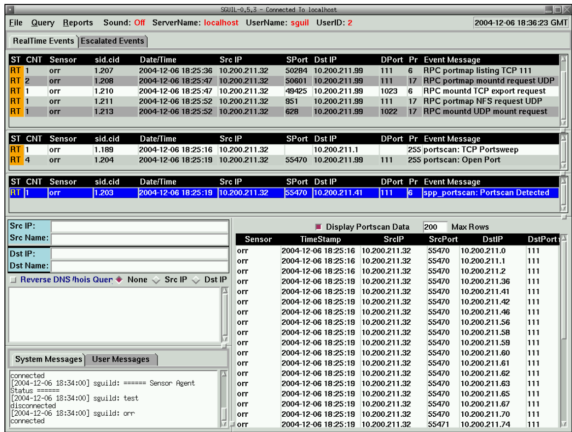
Figure 10: Sguil Port Scan
