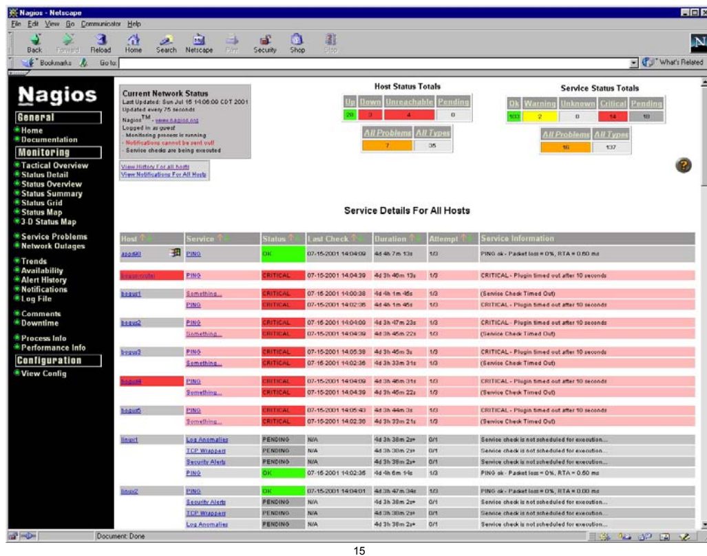
Figure 3: Status Detail (screenshot from Nagios console)
