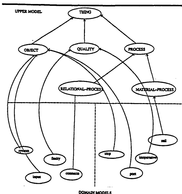
Figure 3: Upper model organization reuse with differing domains
