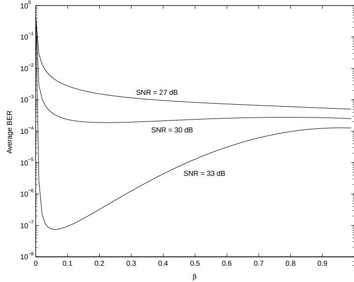
Fig. 7. Average BER as a function of \beta , for different SNR values.
