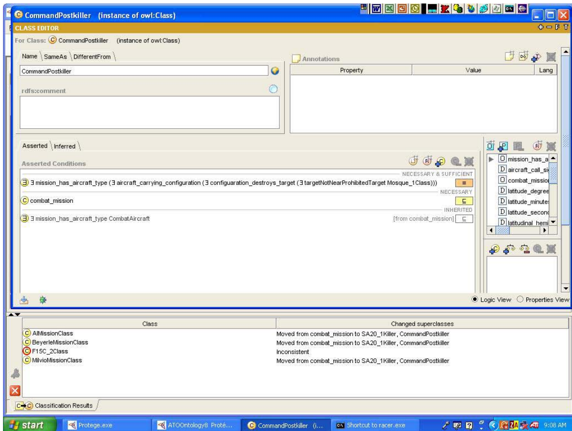
Figure 6 Reasoning on the Knowledge Base
