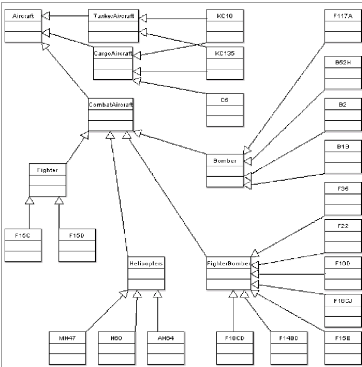
Figure 2 Aircraft Ontology
