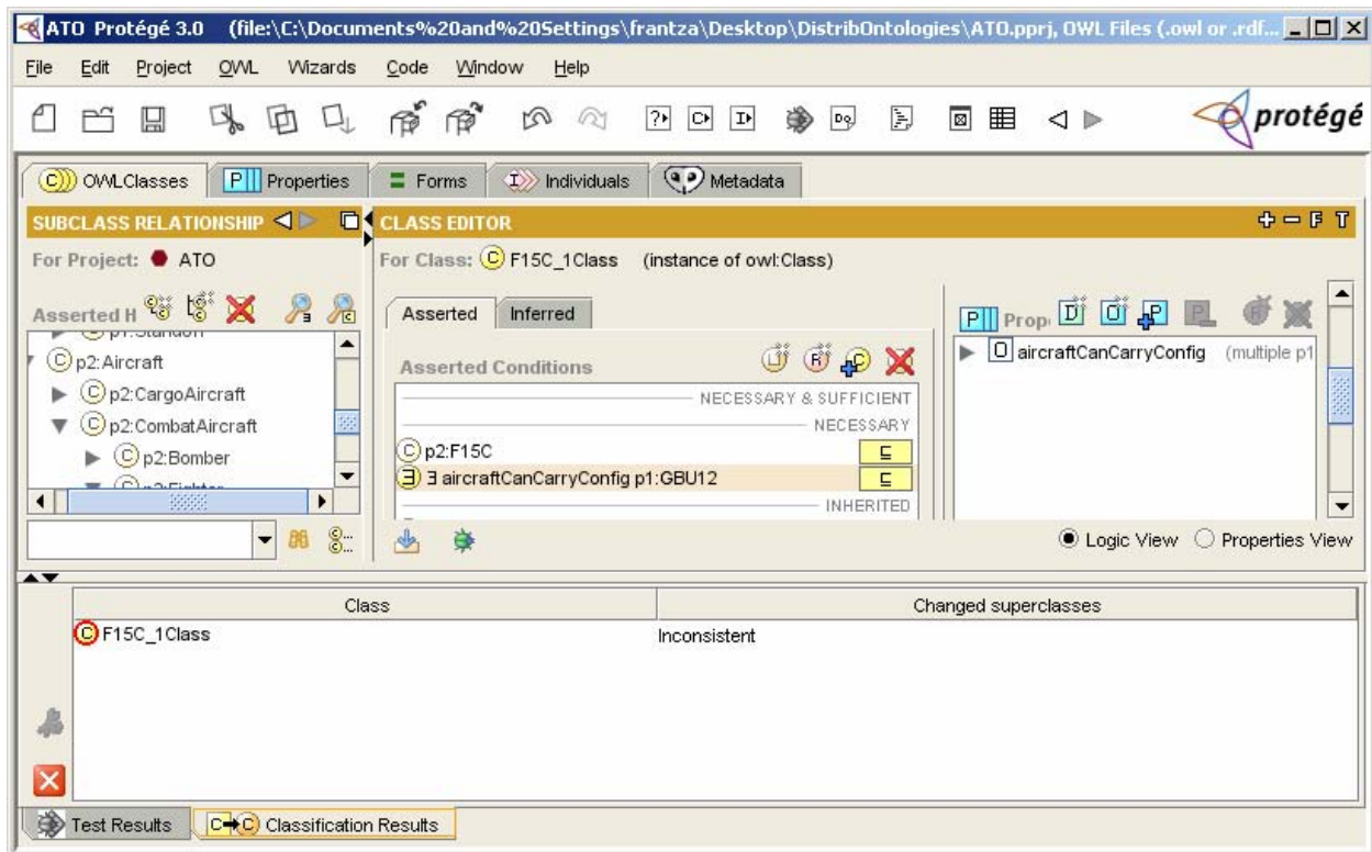
Figure 5 Constraint Violation
