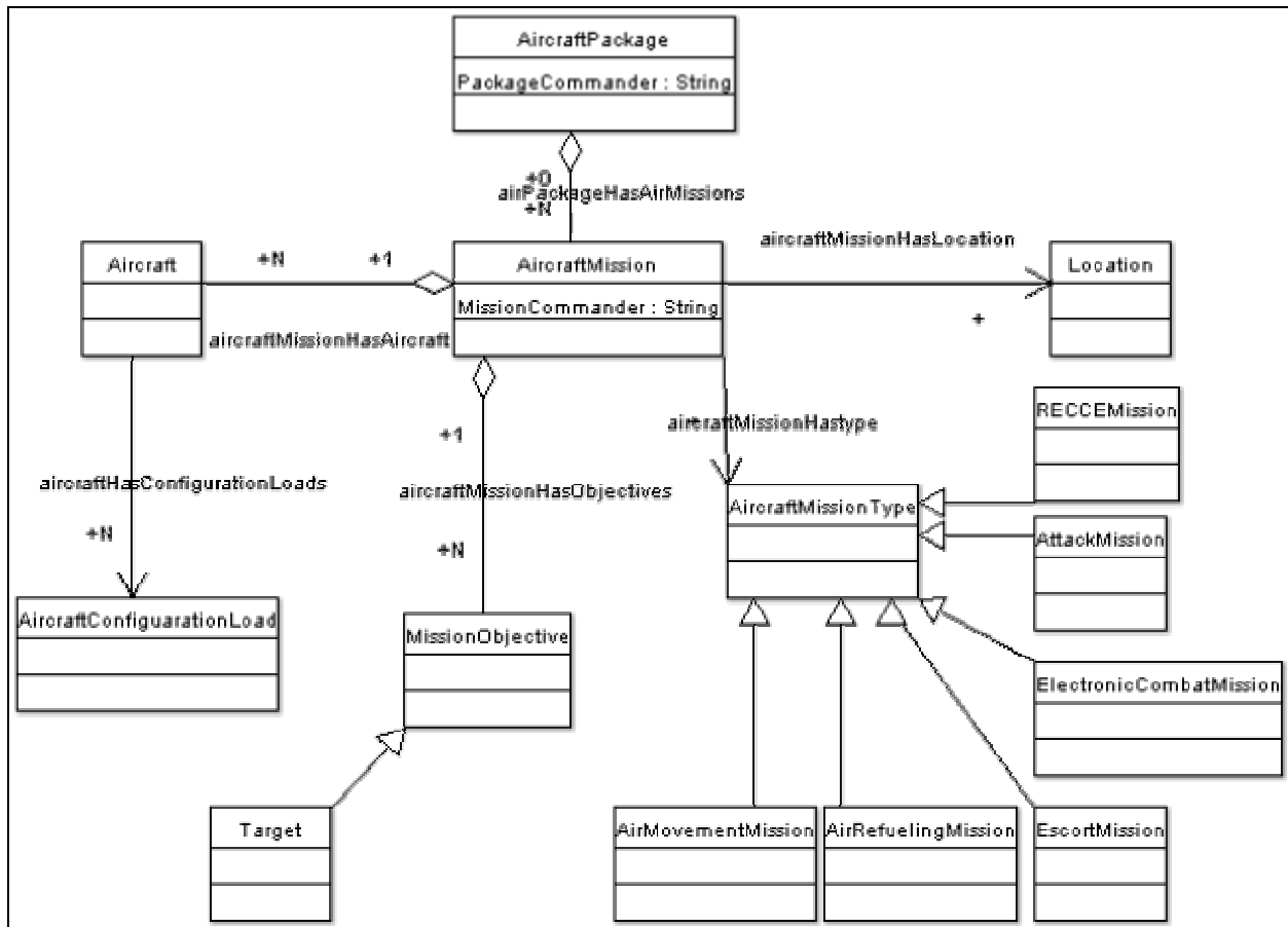
Figure 3 Aircraft Mission Ontology
