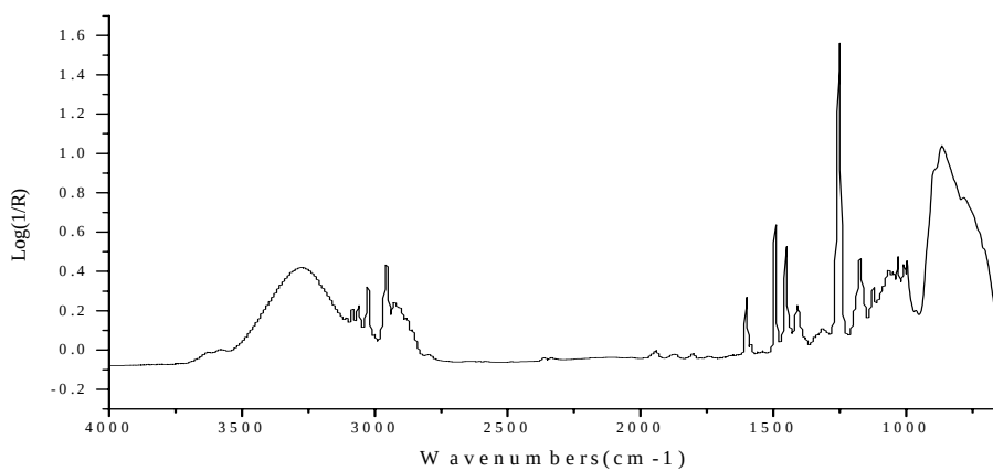
A-5. An infrared spectrum of phenyltrimethylsilanol
