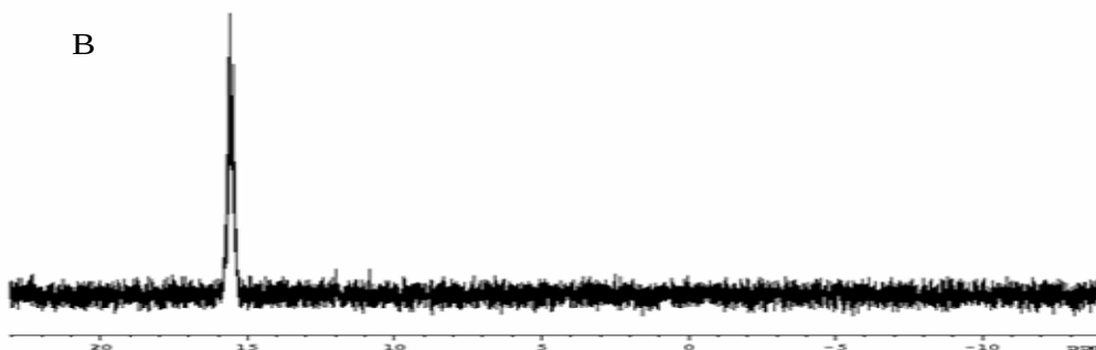
A-9. NMR spectra of n-propyldimethylsilanol, A is H-1 NMR, B is Si-29 NMR in Benzene-D 6 solvent.
