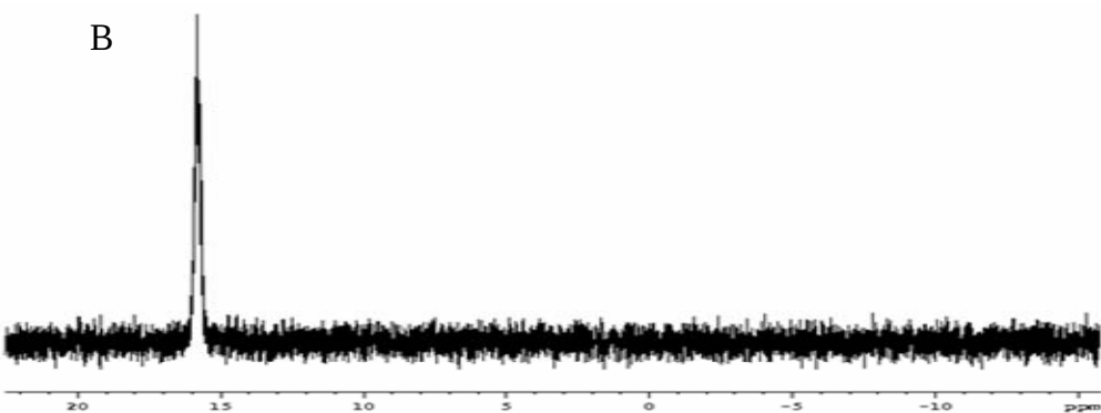
A-10. NMR spectra of n-butyldimethylsilanol, A is H-1 NMR, B is Si-29 NMR in Benzene-D 6 solvent.
