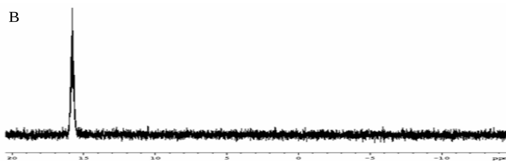
A-15. NMR spectra of pentyldimethylsilanol, A is H-1 NMR, B is Si-29 NMR in Benzene-D 6 solvent
