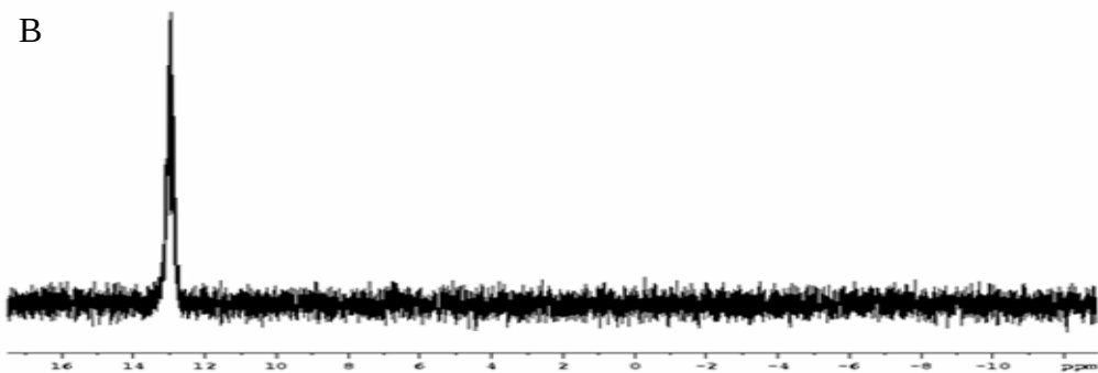
A-11. NMR spectra of bezyldimethylsilanol, A is ^1\text{H} NMR, B is ^{29}\text{Si} NMR in Benzene- \text{D}_6 solvent.
