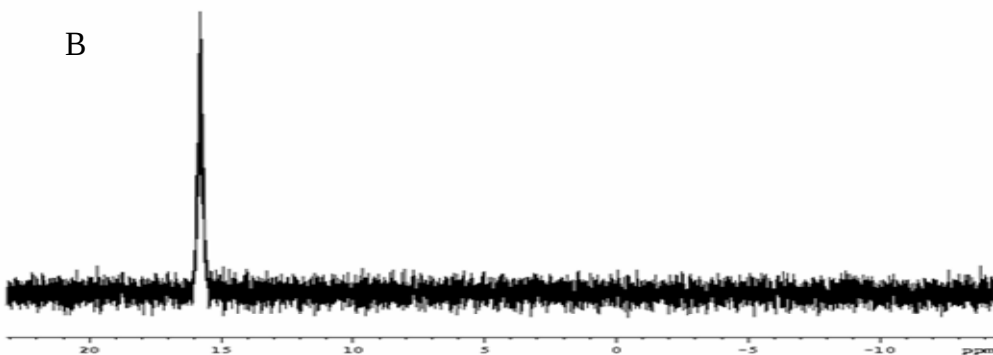
A-16. NMR spectra of hexyldimethylsilanol, A is H-1 NMR, B is Si-29 NMR in Benzene-D 6 solvent.
