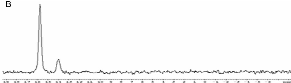
A-12. NMR spectra of phenethyldimethylsilanol, A is ^1\text{H} NMR, B is ^{29}\text{Si} NMR in Benzene- \text{D}_6 solvent
