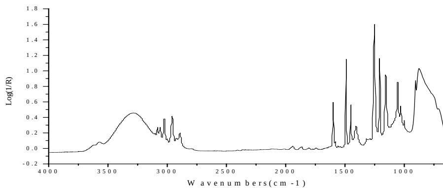
A-4. An infrared spectrum of benzyltrimethylsilanol
