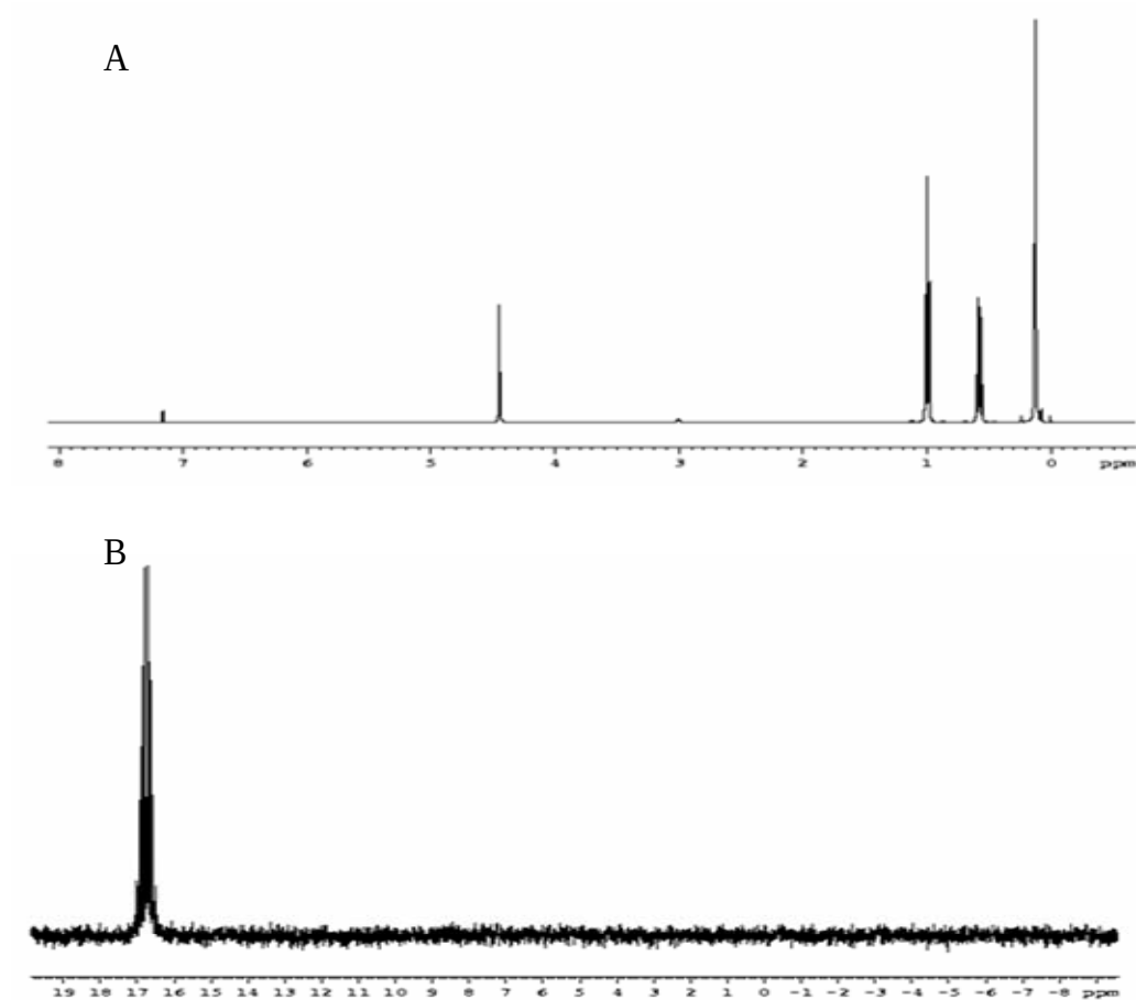
A-8. NMR spectra of ethyltrimethylsilanol, A is 1 H NMR, B is 29 Si NMR in Benzene- 6 D 6 solvent.
