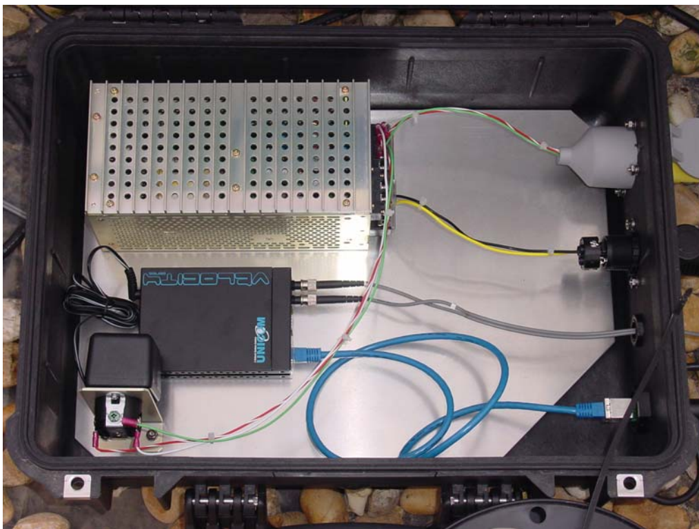
Figure 4. Internal configuration of re-designed conversion box.
