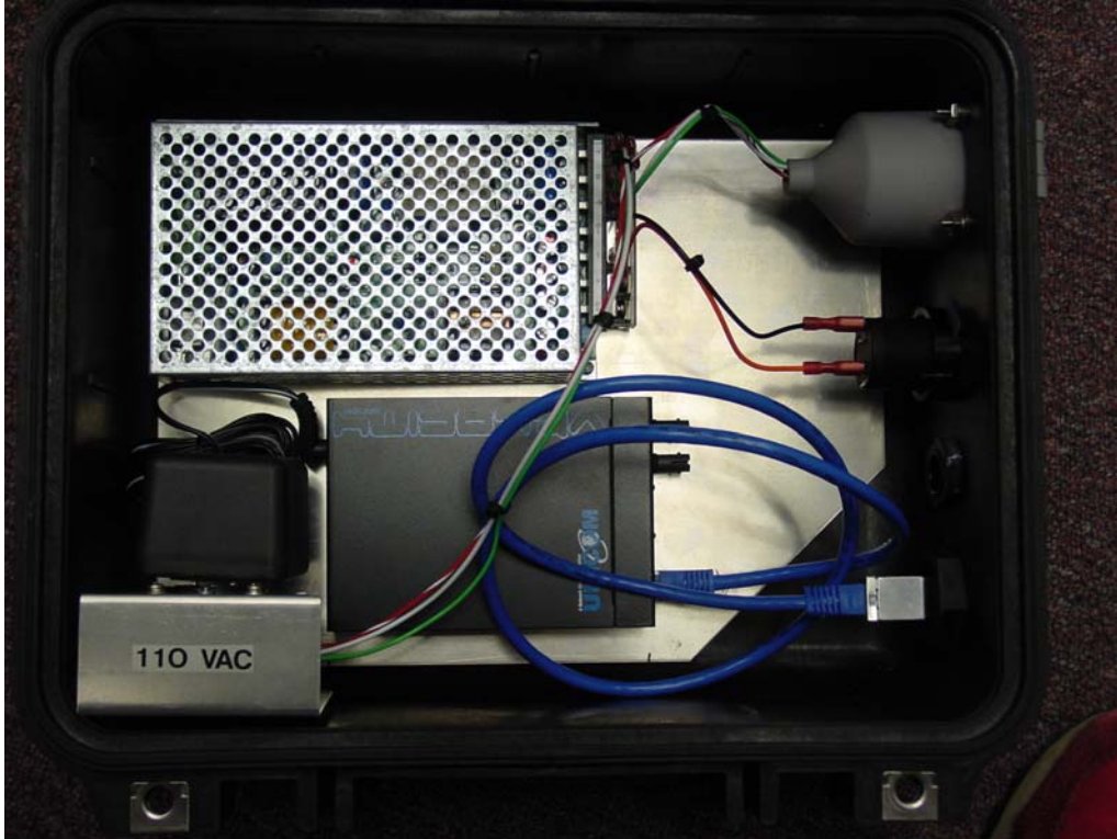
Figure 2. Internal configuration of conversion box.
