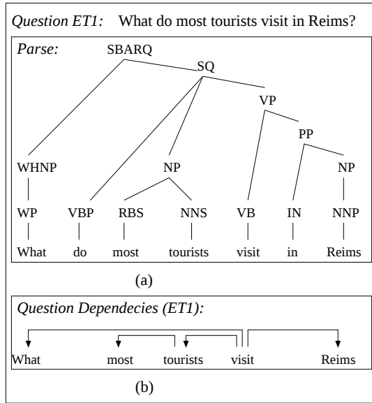
Figure 1: Example of TREC test question
