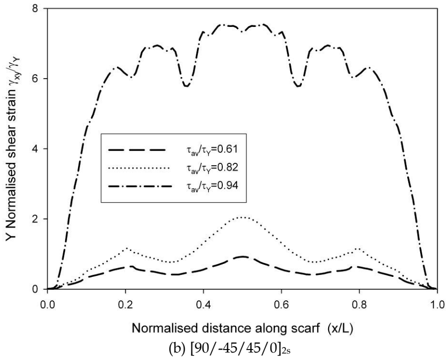
Figure 9 Shear strain distribution along scarf (shear strain normalised by yield strain for (a) [0/45/-45/90]_{2s} and (b) [90/-45/45/0]_{2s} )
