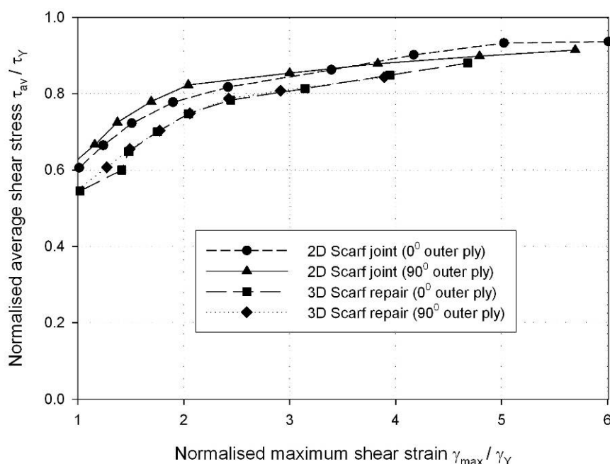
Figure 15 Average shear stress versus maximum shear strain for scarf repair at the highest load location
