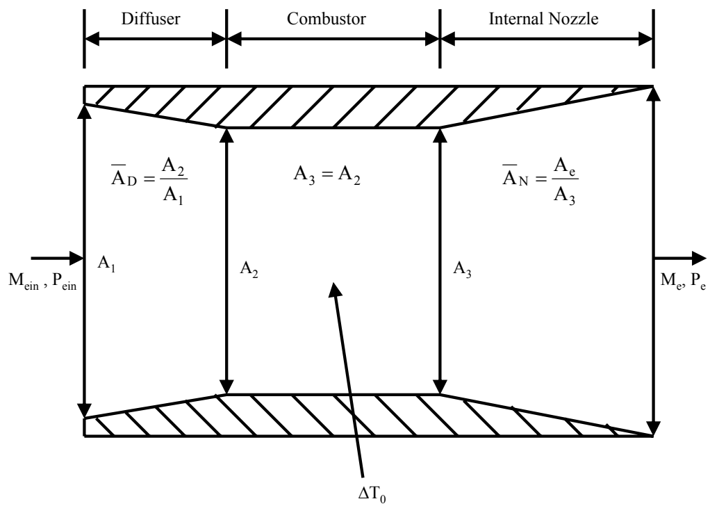
Figure 4. Scramjet Engine.
