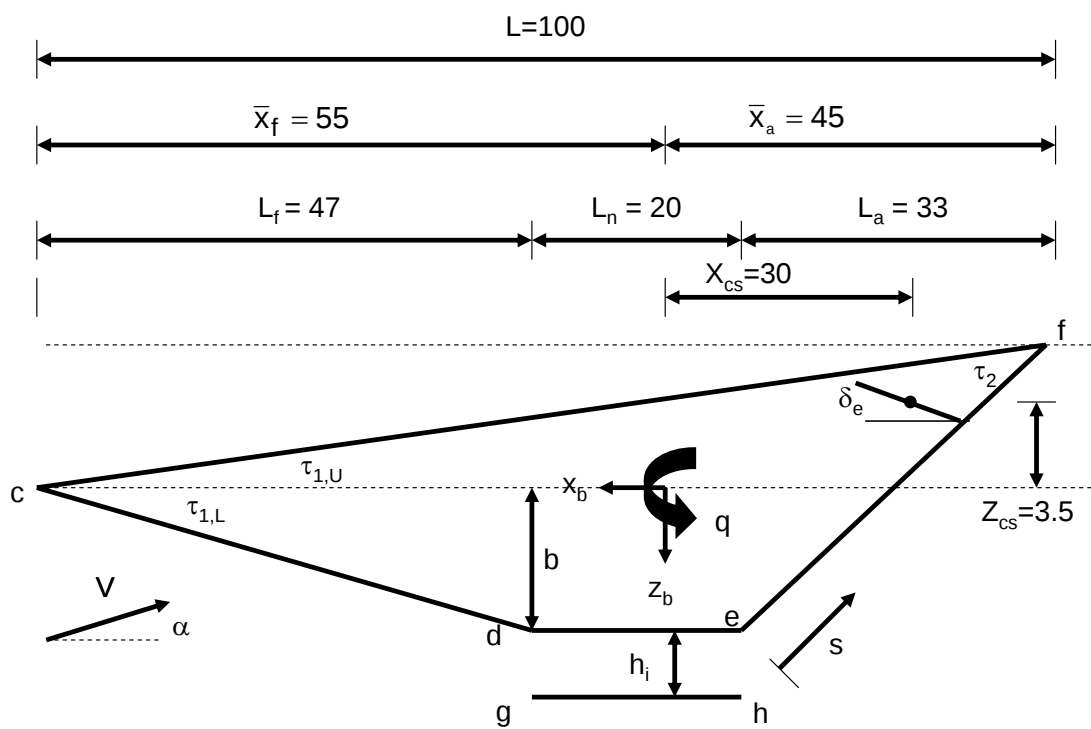
Figure 1. Hypersonic Vehicle.
