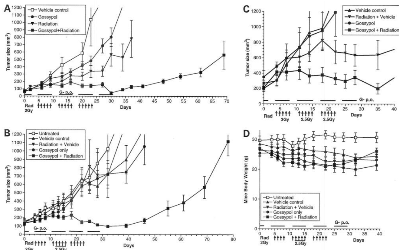
Figure 3. (–)Gossypol [G(–)] in combination with radiation achieves tumor regression in androgen-independent prostate cancer PC-3 xenograft model. PC-3 xenograft tumor growth curves after treatment with fractionated X-ray irradiation and G(–), alone or in combination, where the tumor sizes at the start of G(–) treatment are around 75 mm 3 (A), 150 mm 3 (B), and 230 mm 3 (C). PC-3 cells ( 5 \times 10^6 ) were s.c. injected into the lower back above the tail of each mouse, both sides. When tumors reached appropriate size, the mice were randomized into five to eight mice per group and treated with either G(–) 10 mg/kg p.o., q.d. \times 5 , \times 4 weeks; or X-ray irradiation 2 to 3 Gy, q.d. \times 5 , \times 3 weeks, or their combination. Vehicle control group and radiation only group received same amount of 10% ethanol which is solvent for G(–). The average tumor sizes were shown ( n = 10-16 ). The total radiation doses were 30 Gy for A and B, and 40 Gy for C. D, mice body weights from experiment B during treatment were plotted. (–)Gossypol in combination with radiation seems not to have significant toxicity as compared with either treatment alone or vehicle control.
