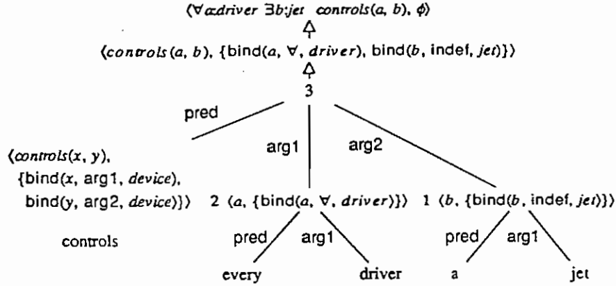
Figure 6: \exists V Interpretation
