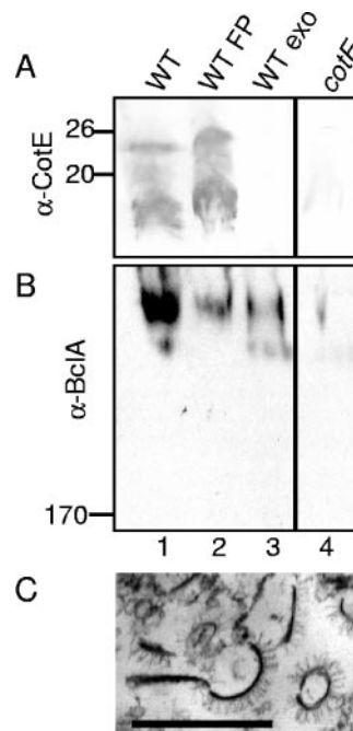
FIG. 6. Subcellular localization of CotE in Sterne strain spores. Spore proteins from wild-type (WT) (strain RG1) (lanes 1 to 3) or cotE mutant (strain RG56) (lane 4) spores were fractionated by SDS-PAGE and subjected to Western blot analysis using anti-CotE (A) or anti-BclA (B) antibodies. Lanes: 1, intact wild-type spores; 2, French-pressed wild-type spores; 3, wild-type exosporium fraction; 4, intact cotE spores. Molecular masses in kDa are indicated on the left. Thin-section electron microscopy was used to verify the purity of the exosporium fraction (C). The size bar indicates 500 nm.
