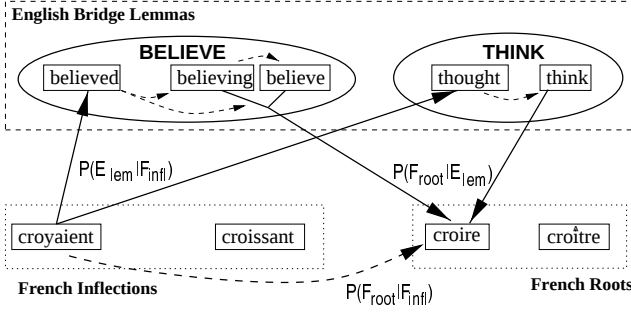
Figure 8: Multi-bridge French inflection/root alignment
