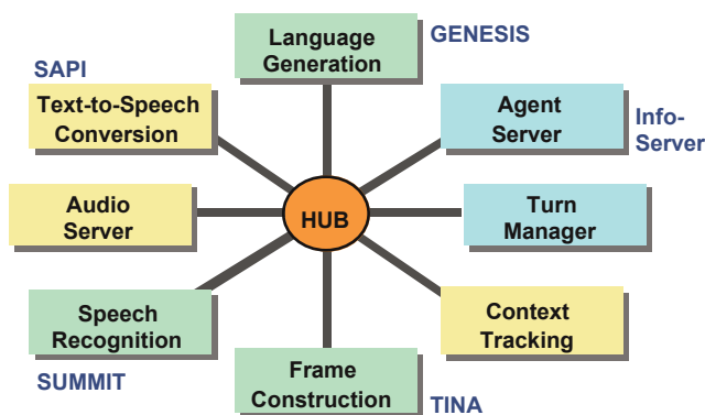
Figure 1. The LCS-Marine architecture.
