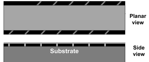
Fig. 5. A YBCO coated conductor that being prepared for transposed multifilamentary structure. An intervening insulation layer is deposited on the structure depicted in Fig. 4. This layer must provide an epitaxial template for subsequent YBCO deposition.
