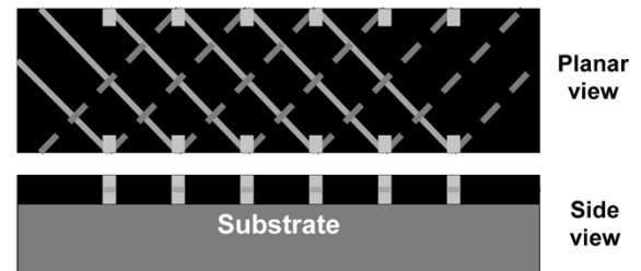
Fig. 6. A YBCO coated conductor that being prepared for transposed multifilamentary structure. A new YBCO layer is deposited on the structure given in Fig. 5 and striations are made into the new YBCO layer separating the filaments on top. The underlying filaments (separated by dashed lines) are connected to the overlying filaments at the edges of the conductor. Current flows in the c-axis direction in YBCO at the edges.
