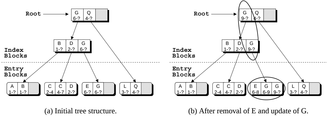
Figure 3: Multiversion b-tree. This figure shows the layout of a multiversion b-tree. Each entry of the tree is designated by a \langle \text{user-key}, \text{timestamp} \rangle tuple which acts as a key for the entry. A question mark (?) in the timestamp indicates that the entry is valid through the current time. Different versions of an entry are separate entries using the same user-key with different timestamps. Entries are packed into entry blocks, which are tracked using index blocks. Each index pointer holds the key of the last entry along the subtree that it points to.
