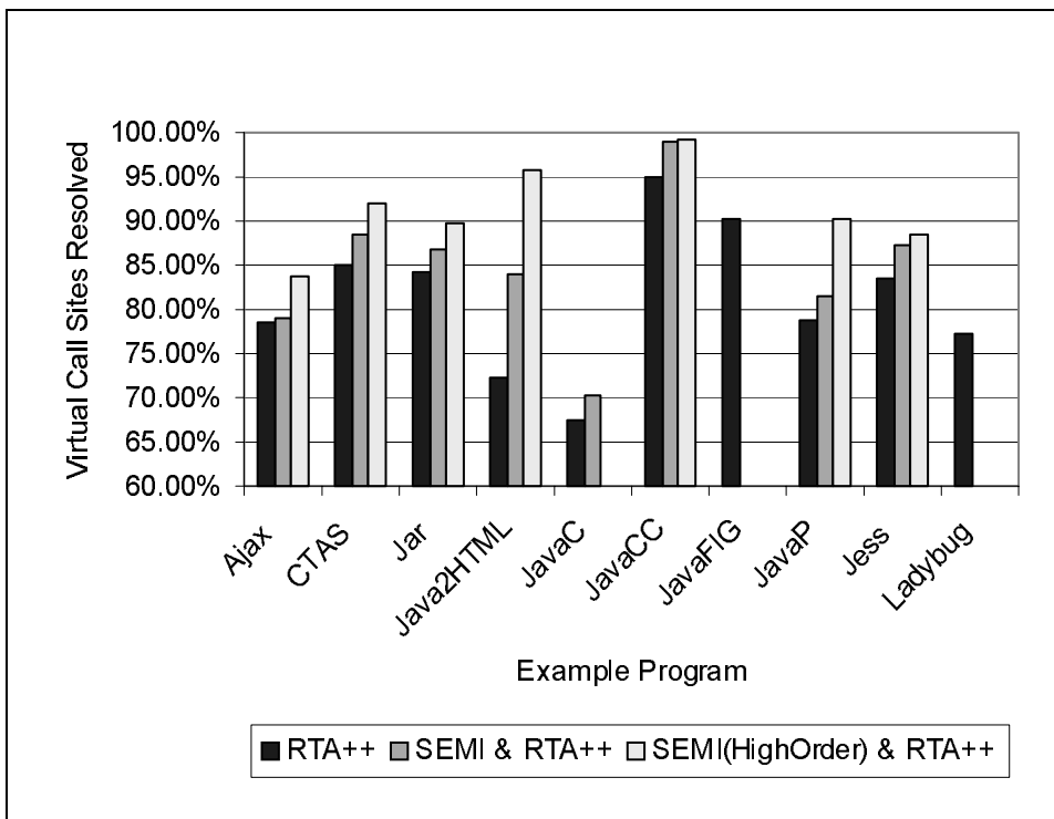
Figure 9-22. Accuracy of the three contending algorithms
