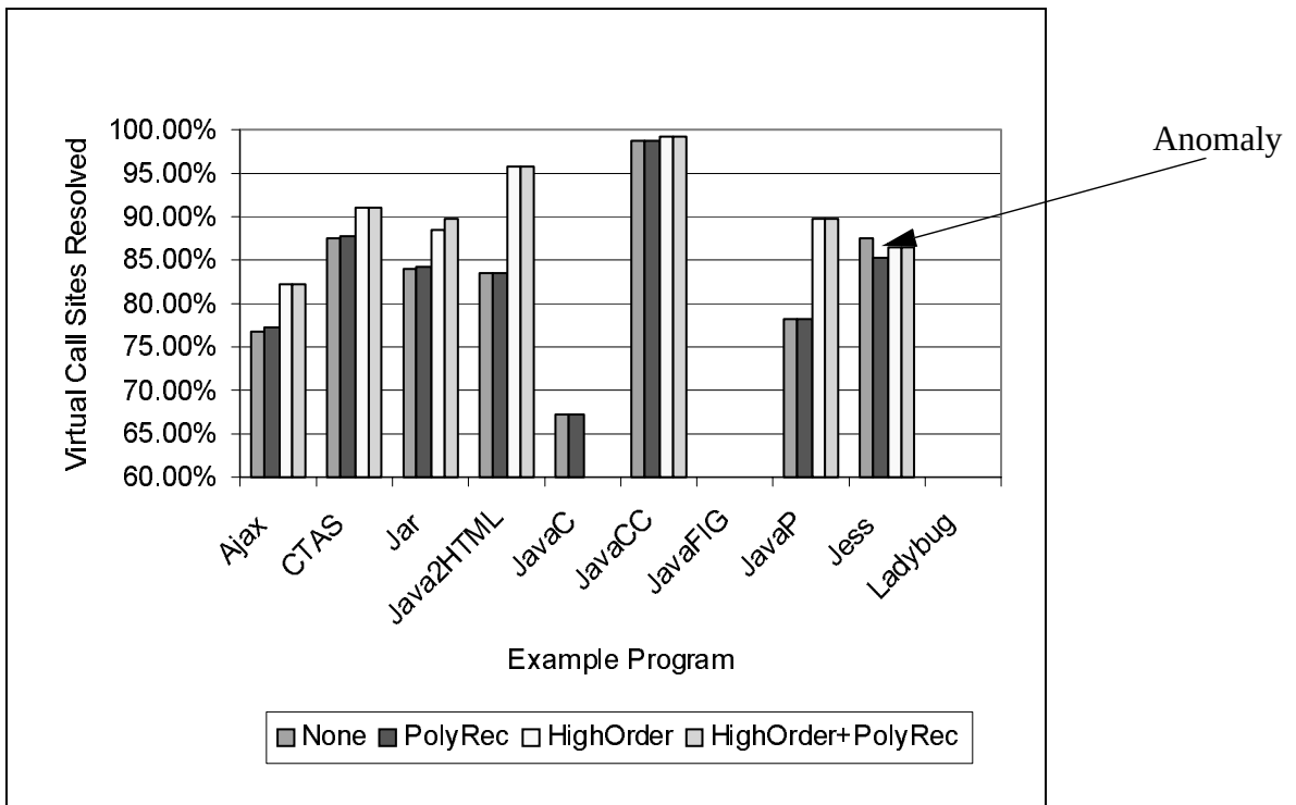
Figure 9-13. Accuracy of SEMI configurations for virtual method call resolution
