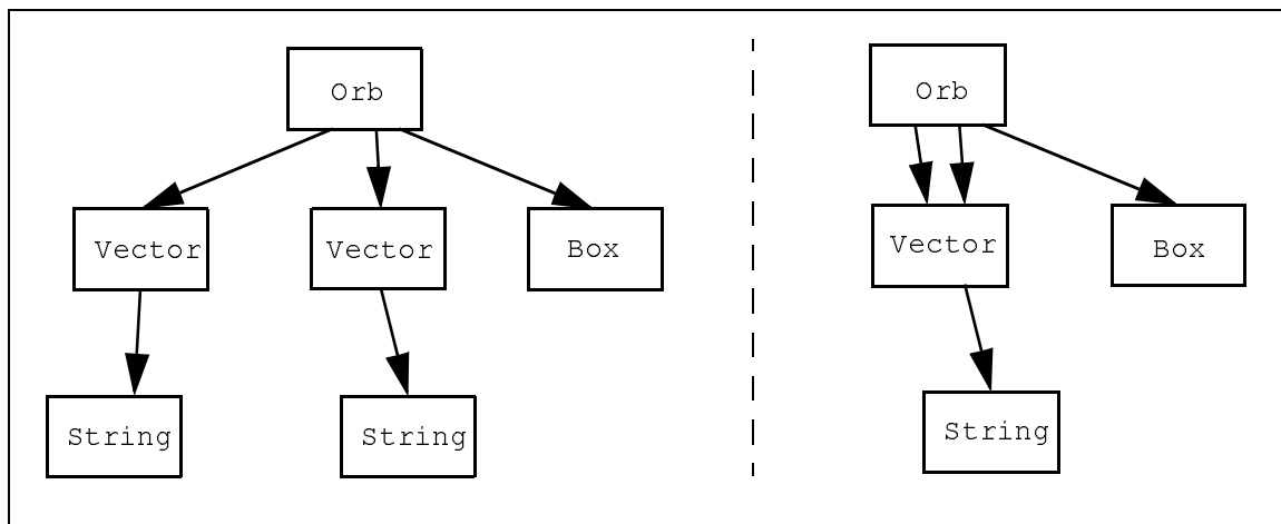
Figure 11-13. Example of merging duplicate subgraphs
