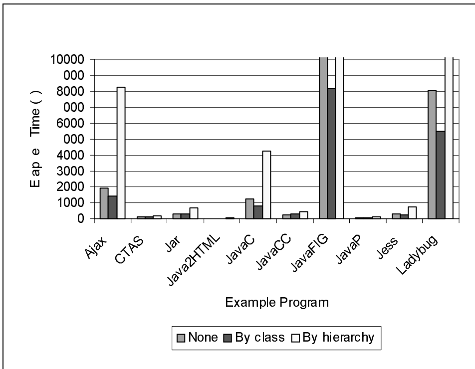
Figure 9-15. Time consumption for different component partitioning schemes
