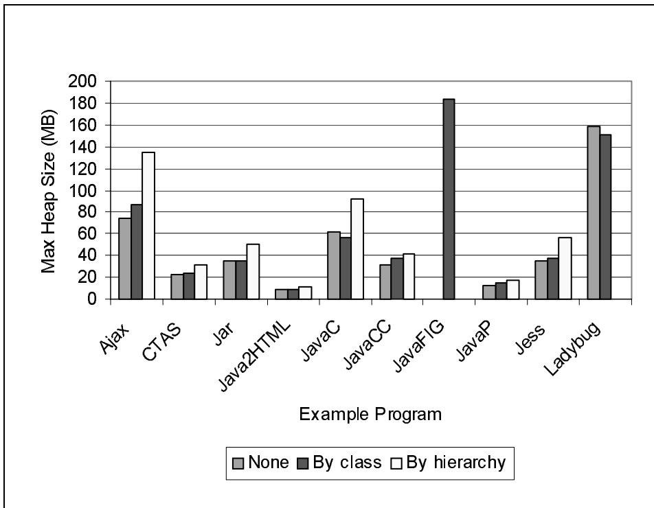
Figure 9-14. Memory consumption for different component partitioning schemes
