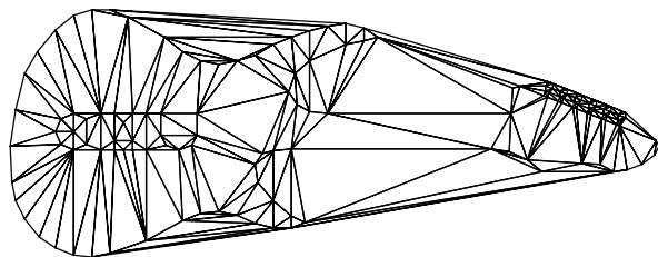
Figure 5.11: Constrained Delaunay triangulation of PSLG.
