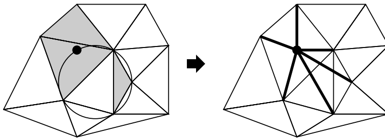
Figure 2.25: The Bowyer/Watson algorithm may behave nonsensically under the influence of floating-point roundoff error.
