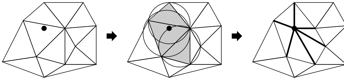
Figure 2.22: The Bowyer/Watson algorithm in two dimensions. When a new vertex is inserted into a triangulation (left), all triangles whose circumcircles contain the new vertex are deleted (center; deleted triangles are shaded). Edges are created connecting the new vertex to the vertices of the insertion polyhedron (right).
