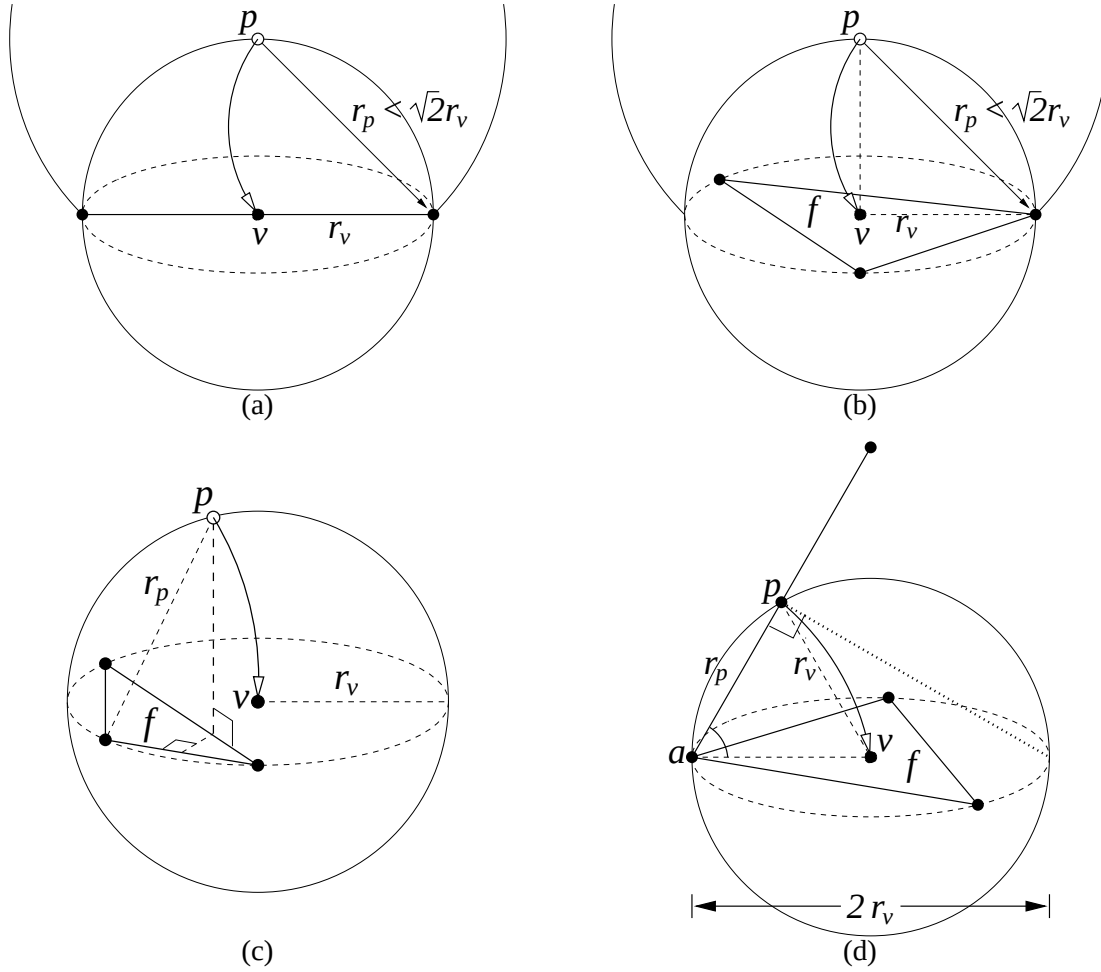
Figure 4.18: The relationship between the insertion radii of a child and its parent. (a) When a subsegment is encroached upon by a circumcenter, the child's insertion radius may be arbitrarily close to a factor of \sqrt{2} smaller than its parent's. (b) When a subfacet that contains its own circumcenter is encroached upon by the circumcenter of a skinny tetrahedron, the child's insertion radius may be arbitrarily close to a factor of \sqrt{2} smaller than its parent's. (c) A bound better than \sqrt{2} applies to a subfacet that does not contain its own circumcenter, but does contain the projection of the encroaching vertex. (d) When a subfacet is encroached upon by the midpoint of a subsegment, and the corresponding facet and segment are incident at one vertex, the analysis differs little from the case of two incident segments.
