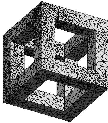
B = 1.04 , \theta_{\min} = 1.01^\circ , \theta_{\max} = 178.21^\circ , h_{\min} = 0.13 , 5884 vertices, 25575 tetrahedra.
