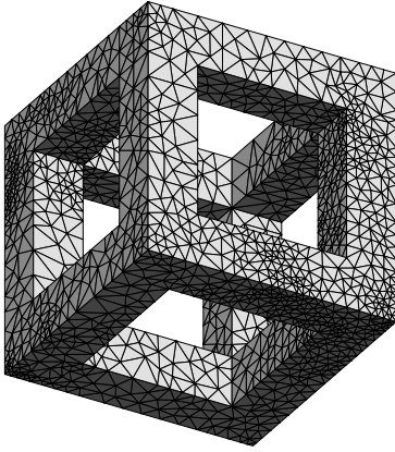
Figure 4.33: Meshes created by Delaunay refinement using equatorial spheres and bounds on both circumradius-to-shortest edge ratio B and smallest dihedral angle \theta_{\min} . Also listed for each mesh is its largest dihedral angle \theta_{\max} and its shortest edge length h_{\min} . The best lower bound on dihedral angles obtained for this PLC is 23.2^\circ . Compare with Figure 4.21 on Page 105.
