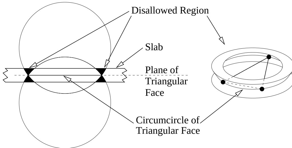
Figure 4.34: Left: A side view of the plane containing a triangular face. In conjunction with this face, a newly inserted vertex can form a sliver with both a small dihedral angle and a small circumradius-to-shortest edge ratio only if it is inserted in the disallowed region (black). Right: An oblique view of the disallowed region of a triangular face.
