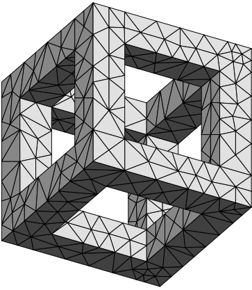
B = 1.2 , \theta_{\min} = 2.01^\circ , \theta_{\max} = 175.89^\circ , h_{\min} = 0.5 , 468 vertices, 1206 tetrahedra.
