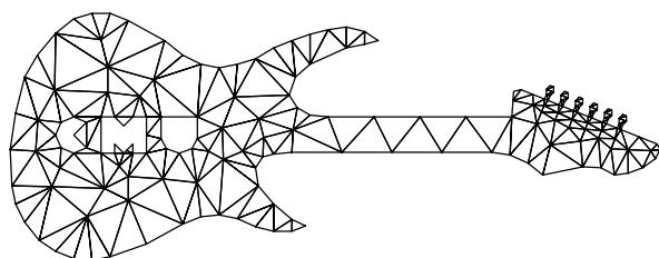
Figure 5.13: Conforming Delaunay triangulation with 20° minimum angle.
