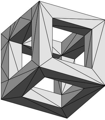
Initial tetrahedralization after segment and facet insertion. 54 vertices, 114 tetrahedra.
