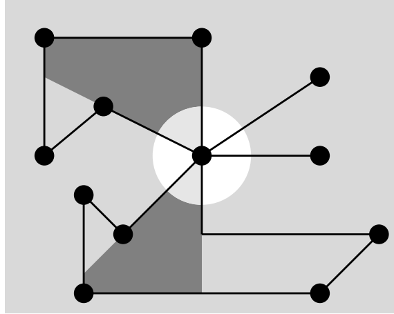
Figure 4.7: In a sufficiently small neighborhood around any vertex, a PLC looks like a set of rays emitted from that vertex.
