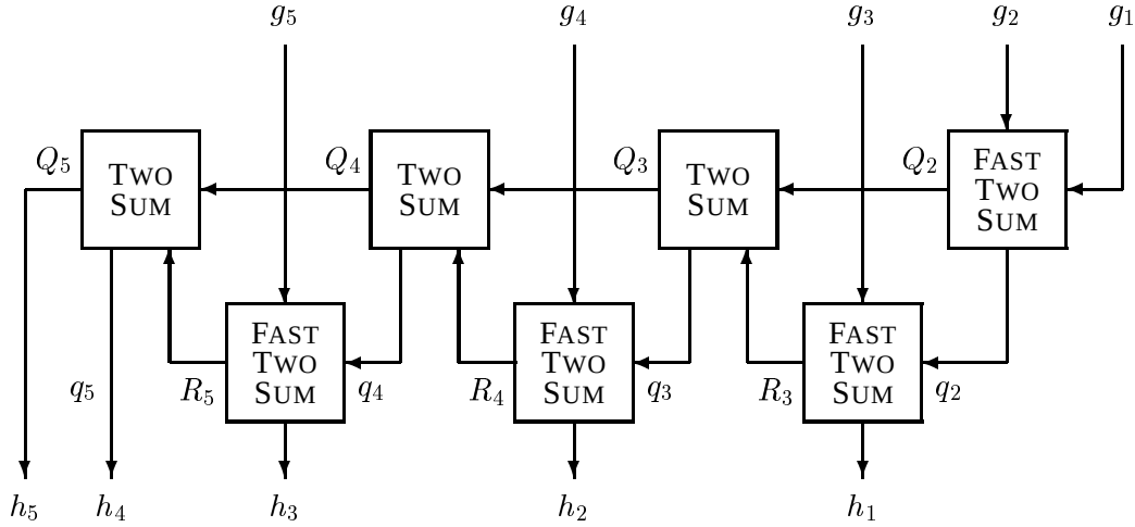
Figure A.1: Operation of LINEAR-EXPANSION-SUM . Q_i + q_i maintains an approximate running total. The FAST-TWO-SUM operations in the bottom row exist to clip a high-order bit off each q_i term, if necessary, before outputting it.
