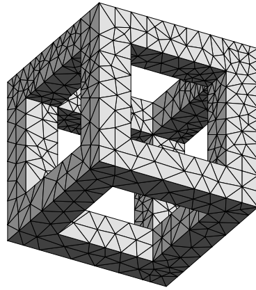
B = 1.1 , \theta_{\min} = 0.69^\circ , \theta_{\max} = 178.83^\circ , h_{\min} = 0.36 , 1135 vertices, 3752 tetrahedra.
