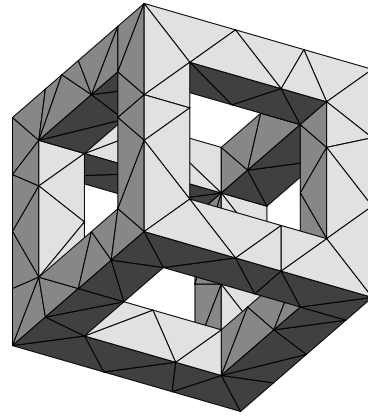
B = 1.4 , \theta_{\min} = 5.42^\circ , \theta_{\max} = 171.87^\circ , h_{\min} = 1.25 , 110 vertices, 211 tetrahedra.
