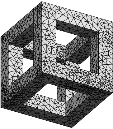
B = 1.05 , \theta_{\min} = 1.01^\circ , \theta_{\max} = 178.21^\circ , h_{\min} = 0.24 , 2997 vertices, 11717 tetrahedra.
