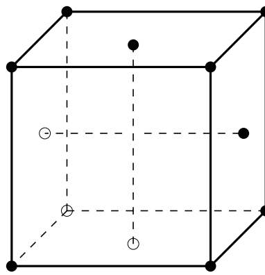
Figure 4.23: A counterexample demonstrating that the three-dimensional Delaunay refinement algorithm is not size-optimal.
