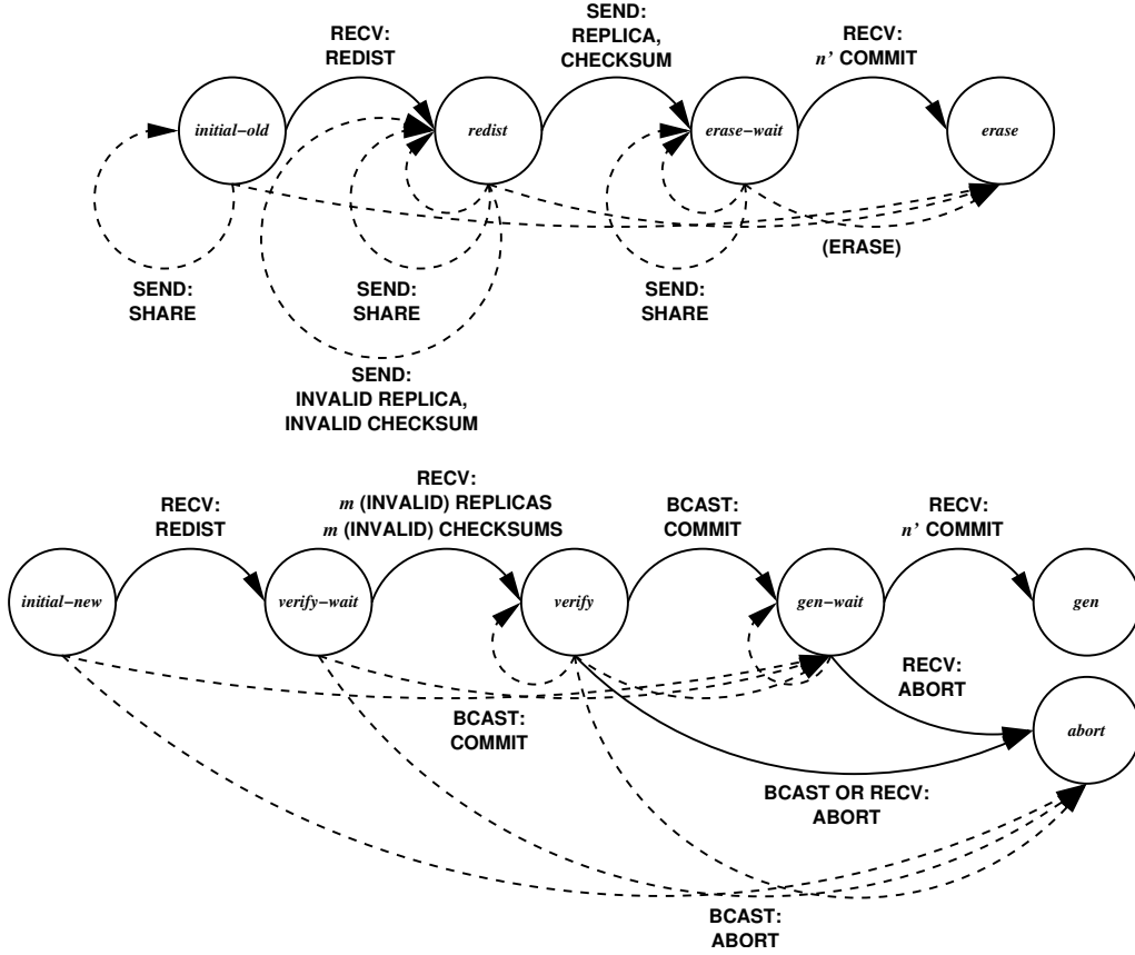
Figure A.1: REDISTRIBUTE state machines for old and new servers, in a system that uses the REPLICA scheme. States correspond to intermediate computations, while state transitions correspond to sent or received messages. Old servers start in the initial-old state. New servers start in the initial-new state. Solid arrows indicate transitions taken by correct servers, while dashed arrows indicate transitions that may be taken by faulty servers. Unlabelled dashed arrows that loop to the same state indicate no-op self-transitions.
