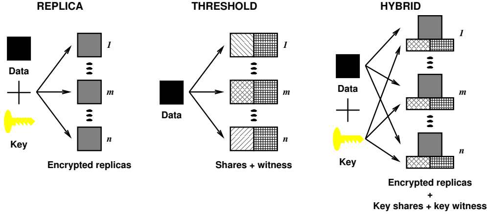
Figure 4.1: REPLICA, THRESHOLD, and HYBRID data distribution schemes implemented in Hathor. In each scheme, n servers store a piece of the original data, and m pieces are required to recover the data. For both REPLICA and HYBRID, the servers store identical encrypted replicas of the data; additionally for HYBRID, the servers store different shares of the encryption key but identical key witnesses. For THRESHOLD, the servers store different shares of the data but identical witnesses to the data. Each replica, data share, and data witness is the same size as the original data; each key share and key witness is the same size as the key.
