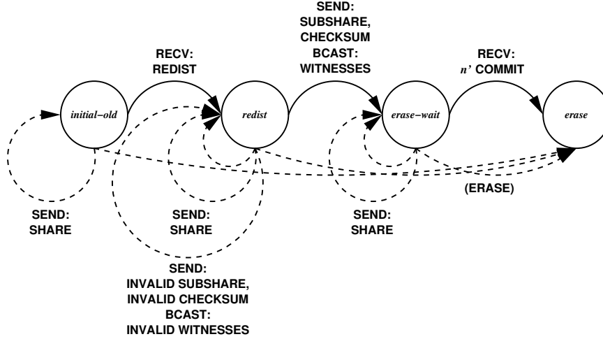
Figure 4.4: REDISTRIBUTE state machine for old servers. States correspond to intermediate computations, while state transitions correspond to sent or received messages. Old servers start in the initial-old state. Solid arrows indicate transitions taken by correct servers, while dashed arrows indicate transitions that may be taken by faulty servers. Unlabeled dashed arrows that loop to the same state indicate no-op self-transitions.
