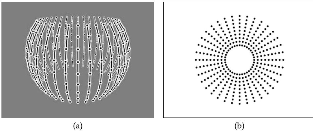
Figure 3.2: A scene consisting of points on longitudinal lines is shown in (a); within each longitudinal line, the points are equally space in angle about the origin. An equiangular omnidirectional camera whose mirror is placed at the origin of the scene images the points at equally spaced positions along the radial lines, as shown in (b).
