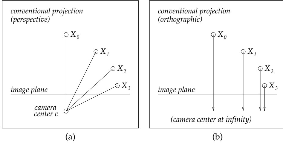
Figure 2.1: Normalized perspective projections are found by intersecting the ray from the scene point to the camera center with the image plane (a). Orthographic projection, which does not model the effects of the scene points' distances from the camera, can be treated as a special case of perspective projection in which the camera center is infinitely far away (b).
