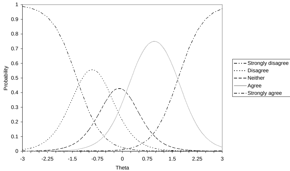
Figure 61. Item characteristic curves for items on Fairness Scale (Q27B: Navy policies retain best quality Sailors).
