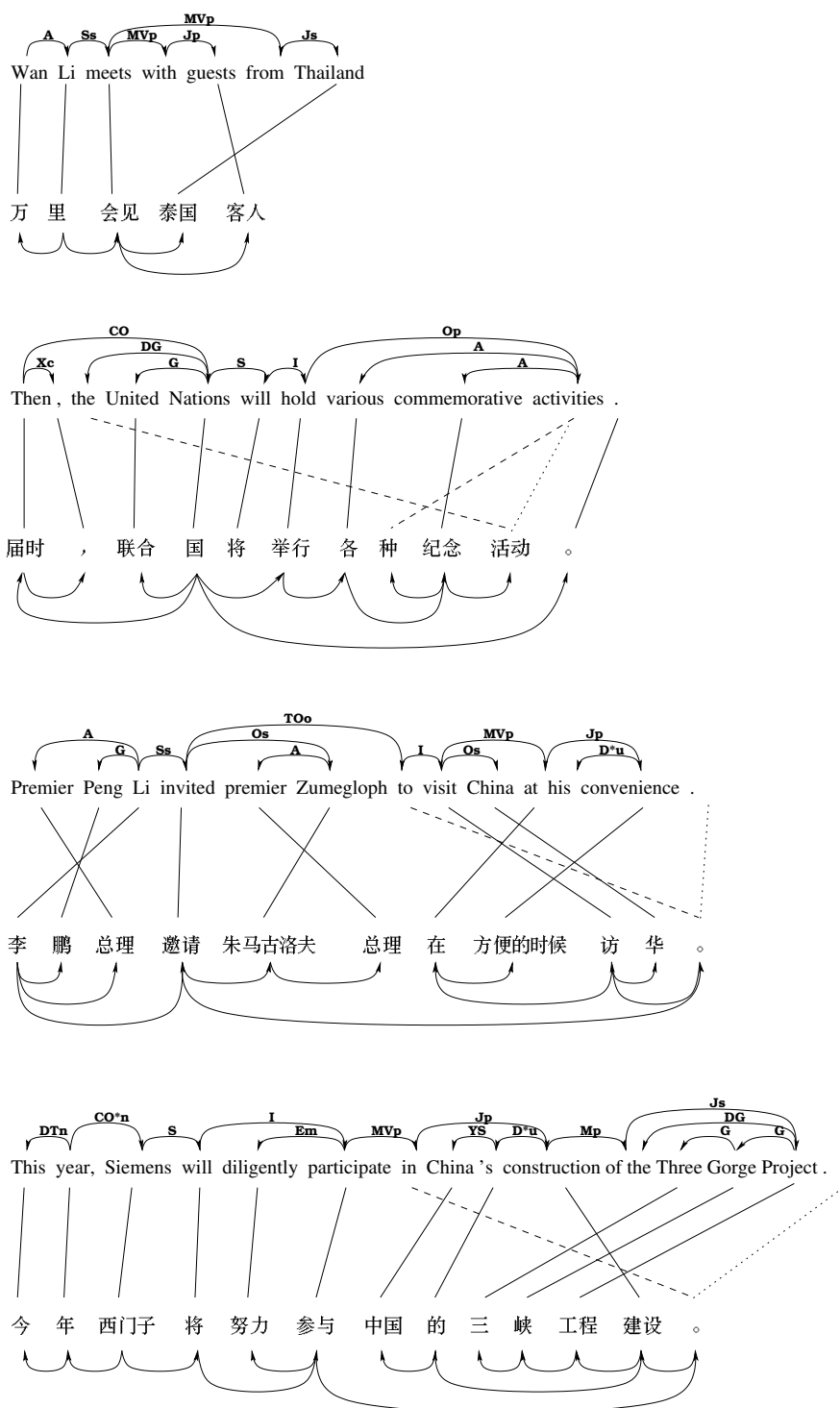
Figure 3.15: Selected Chinese–English sentence pairs aligned with LinkSet.
