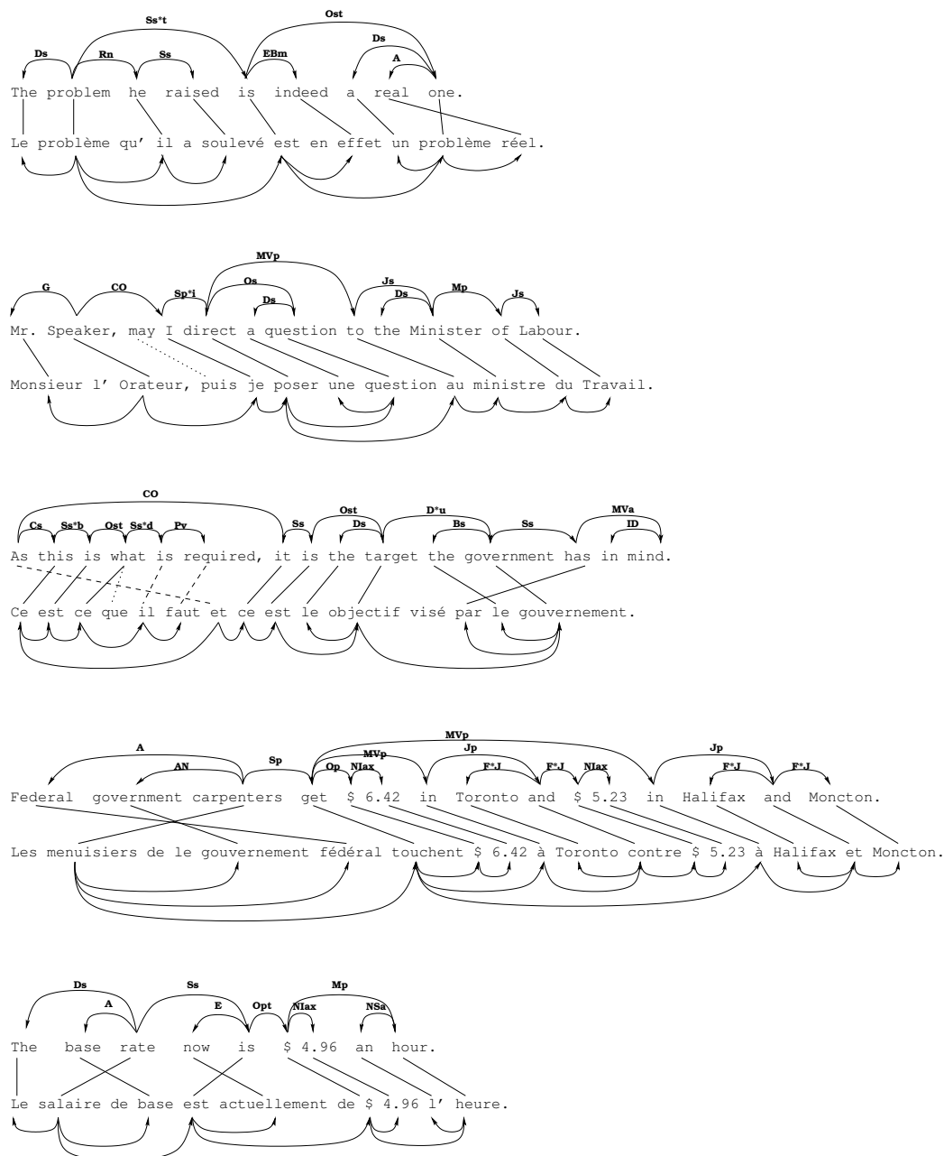
Figure 3.13: Selected French-English sentence pairs aligned with LinkSet.
