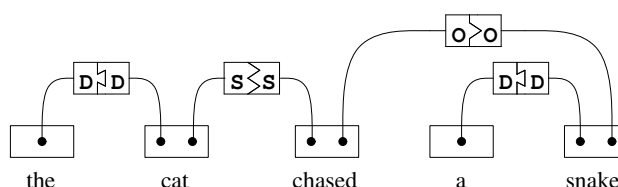
Figure 2.2: A sentence.
