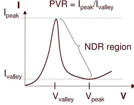
Figure 2: I - V curve for a “typical” RTD device.
