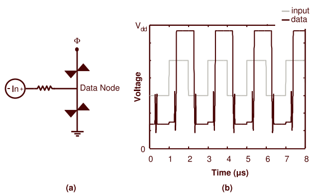
Figure 5: (a) Simple molecular latch circuit used in testing. (b) Results of single stability experiment. Note voltage “gain.” and memory effect.
