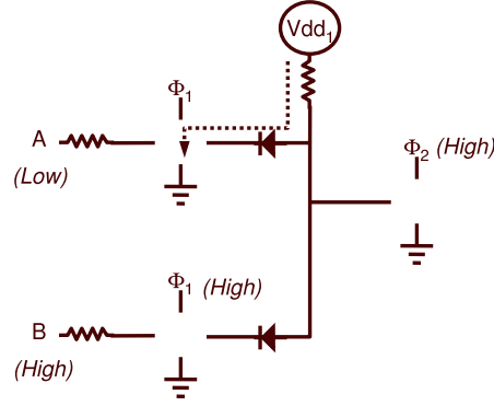
Figure 10: Lack of I/O isolation in AND circuit provides path from V_{dd1} to ground.
