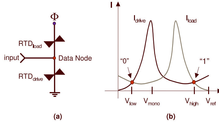
Figure 3: (a) Basic molecular latch configuration. (b) Load-line diagram for molecular latch.
