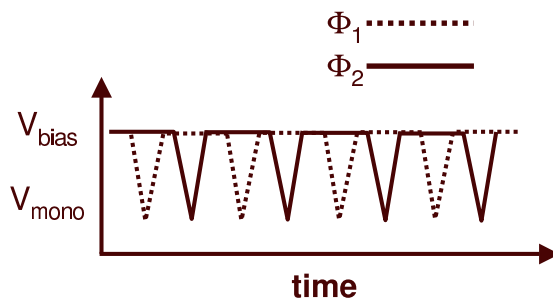
Figure 7: Two-phase clocking scheme used for series latches.
