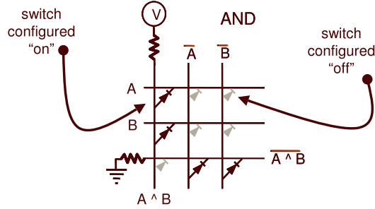
Figure 1: A two-input AND gate implemented in a reconfigurable CAEN grid.
