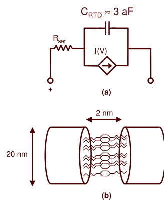
Figure 4: (a) Device model for RTD. (b) Possible construction technique for molecular RTD as an inline device (not to scale).
