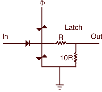
Figure 8: The complete molecular latch.
