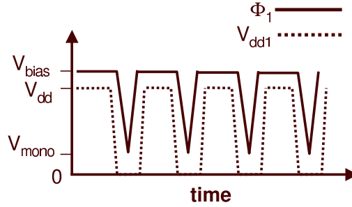
Figure 11: Clocking scheme used for V_{dd} .
