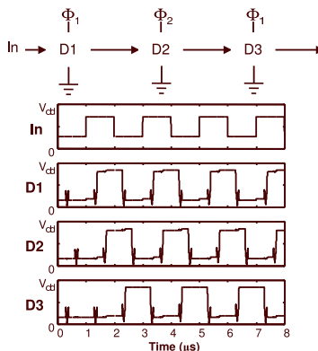
Figure 6: Simple 3-stage delay circuit using molecular latch from Figure 8.
