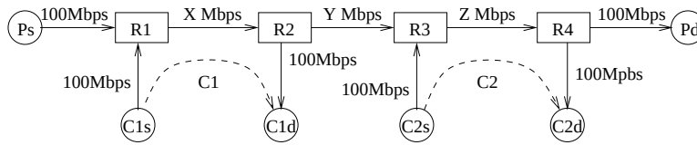
Figure 21: Simulation configuration. Ps , Pd are the hosts used for probing, and C1s , C1d , C2s , C2d are used for the competing traffic generation. The numbers on the links denote the link capacity. The competing traffic flow C1 is the traffic we want to measure. The competing flow C2 is the competing traffic on a non-bottleneck link.
