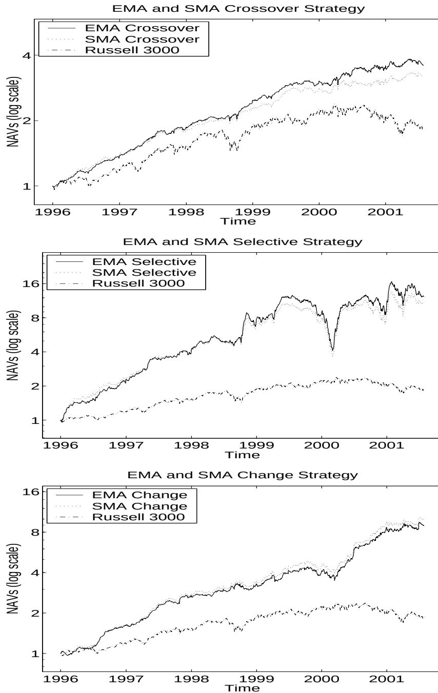
Figure 2.4: Moving Average Strategies NAV Plots
