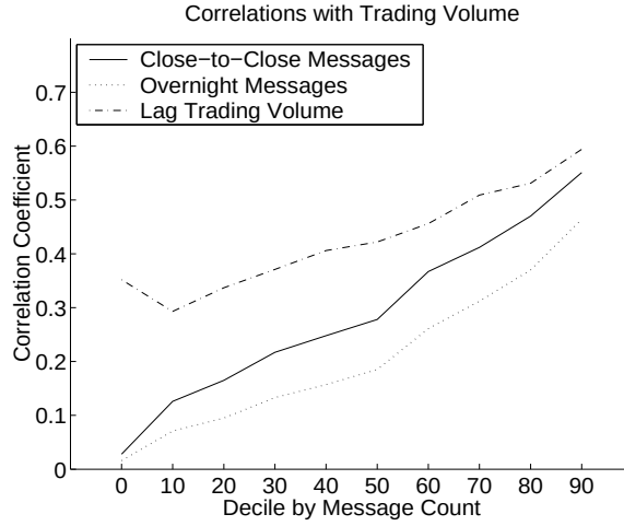
Figure 4.7: Correlations between trading volume and lag trading volume, close-to-close message counts, and overnight message counts
