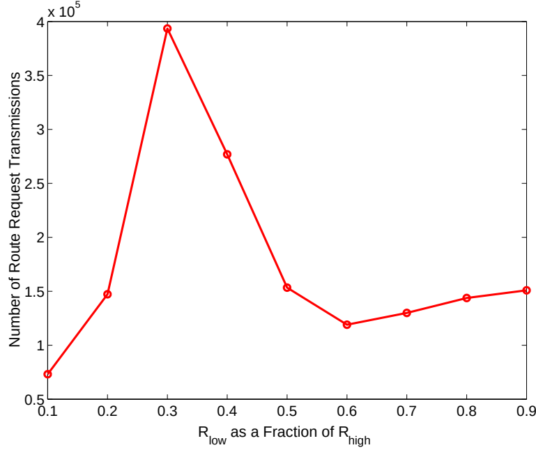
Figure 4.1: Simulation of AODV in mobile ad hoc networks with 10 nodes with transmission range R_{high} = 250\text{m} and 90 with range R_{low} , all moving according to a random waypoint model with 1 m/s maximum speed and 0 pause time. 35 pairs of nodes exchange one-way CBR traffic at four 64-byte packets per second.
