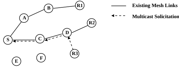
Figure 2.7: Node D receives a source-specific MULTICAST SOLICITATION and unicasts it on to the source.
