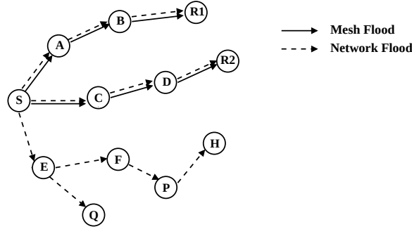
Figure 2.3: Mesh Flood vs. Network Flood.
